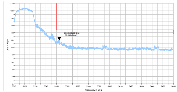
802.11a-Channel 64: Average
