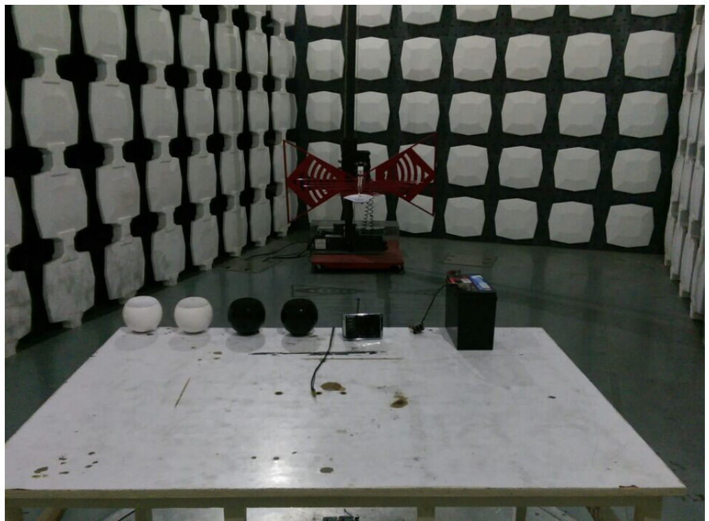
Radiated Emission Test
