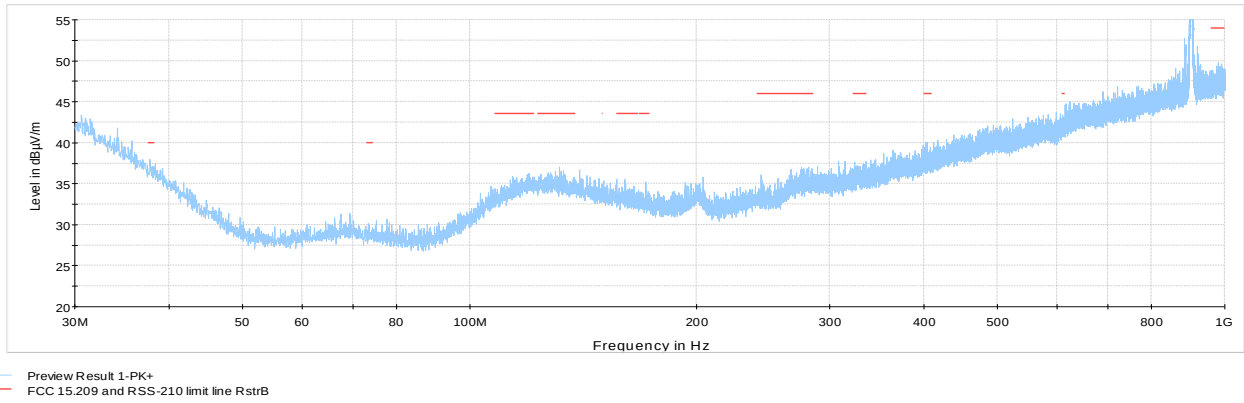
Figure 8.6-8: Radiated spurious emissions 30 MHz–1GHz Tx @ low ch
