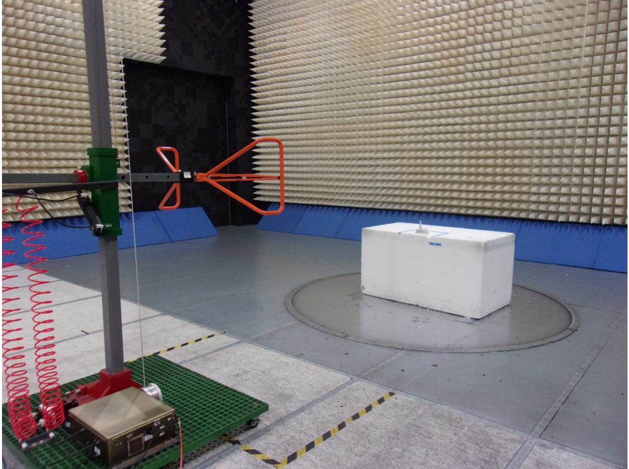
Unintentional Emissions – 30MHz – 1GHz Spurious Emissions – 30MHz – 1GHz
