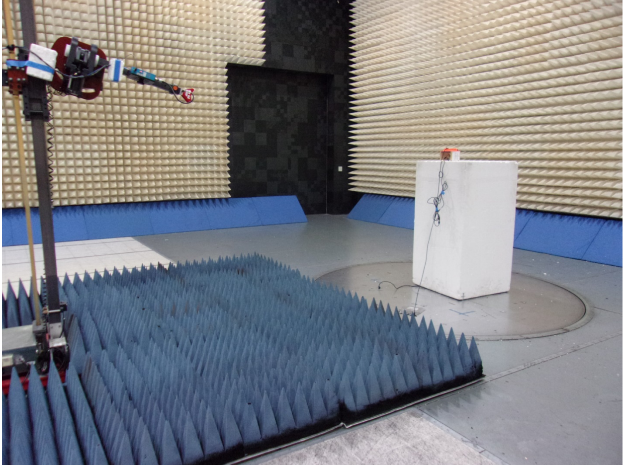
Spurious Emissions – 18GHz – 40GHz
