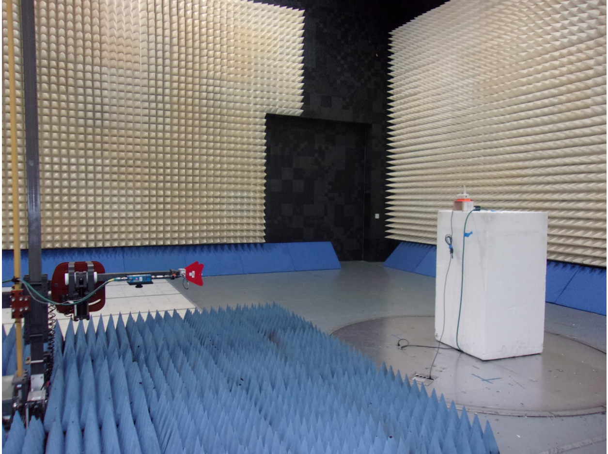
Spurious Emissions – 1GHz – 18GHz
