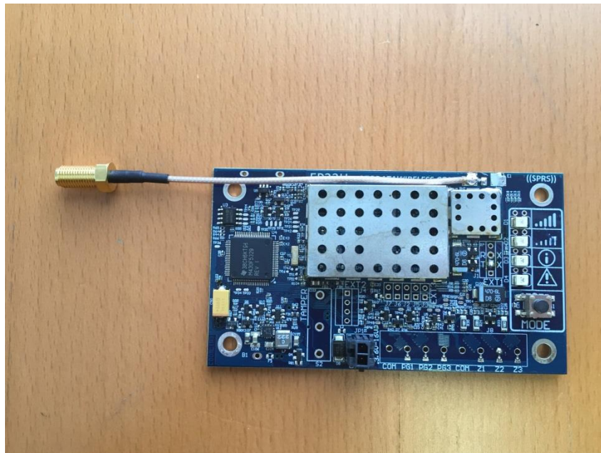
C005 Top PCB with shield and marketed SMA-RP connector
