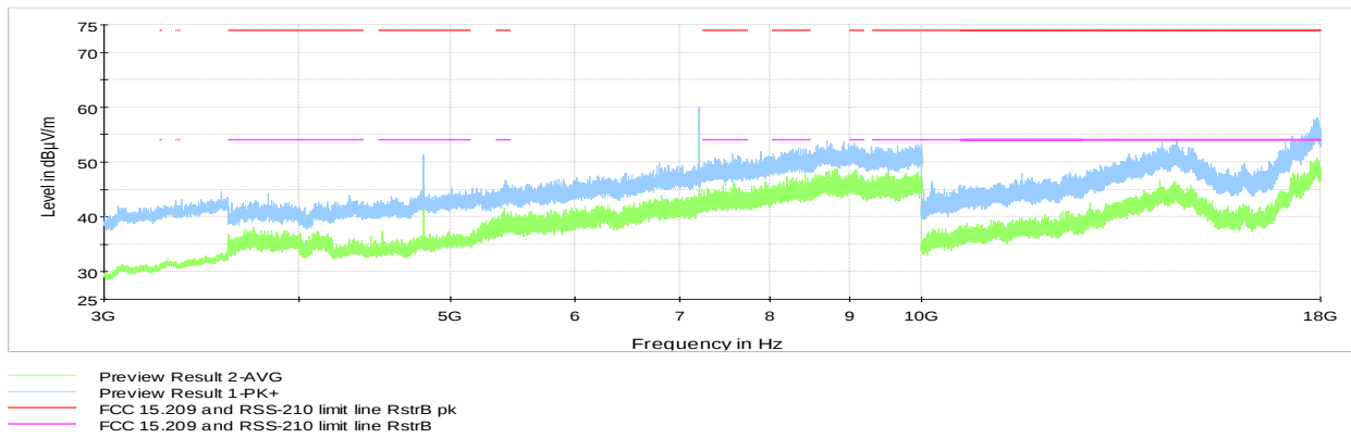
Figure 8.6-12: Radiated spurious emissions 3 to 18GHz, Tx at low channel, variant ES3016
