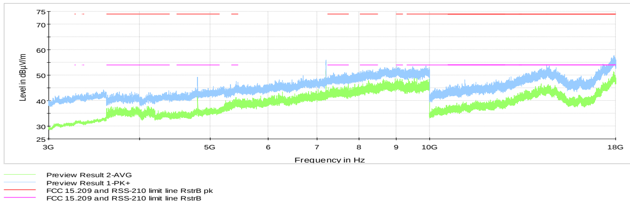
Figure 8.6-18: Radiated spurious emissions 3 to 18GHz, Tx at low channel, variant ES3022
