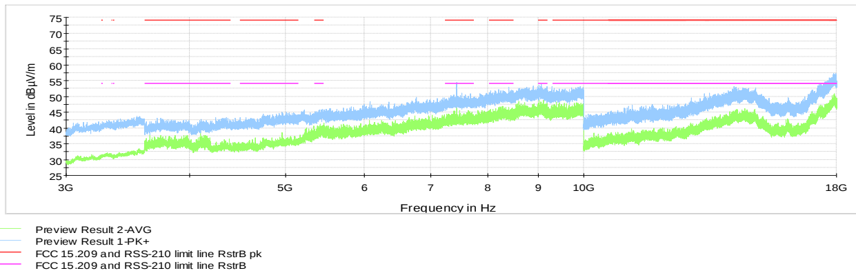
Figure 8.6-26: Radiated spurious emissions 3 to 18GHz, Tx at low channel, variant ES3026
