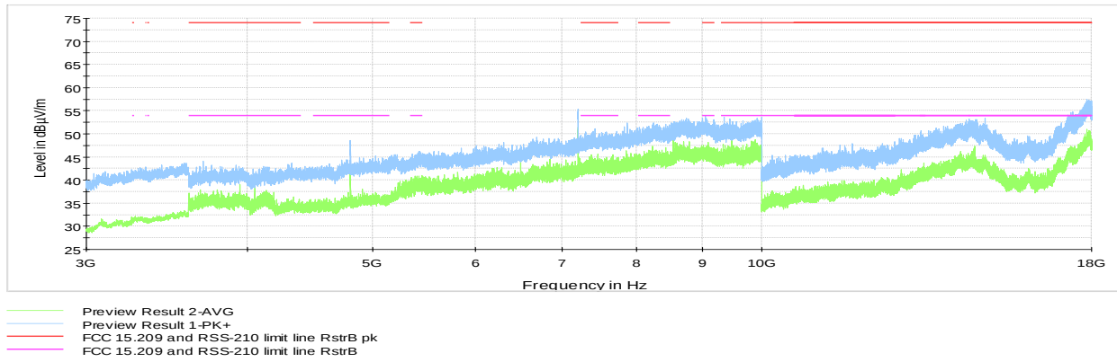
Figure 8.6-24: Radiated spurious emissions 3 to 18GHz, Tx at low channel, variant ES3026
