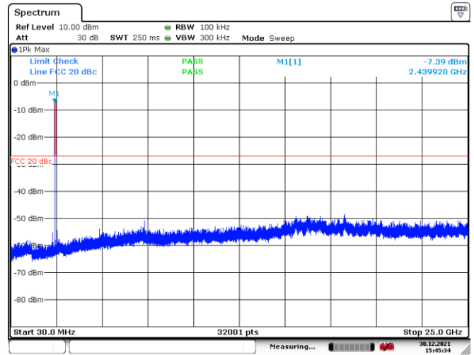
Figure 8.6-2: Conducted spurious emissions Tx on mid channel
