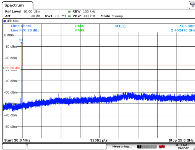
Figure 8.6-1: Conducted spurious emissions Tx on low channel
