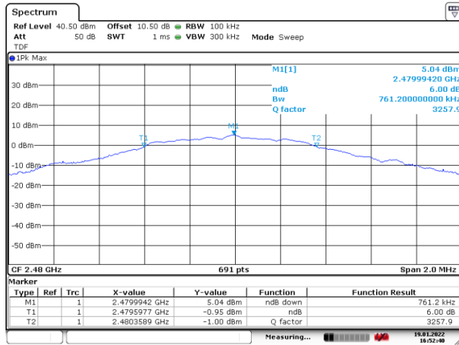
Figure 8.4-3: 6 dB bandwidth on high channel
