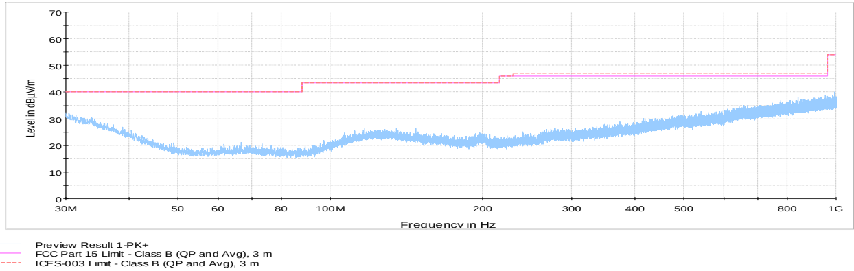
Figure 8.6-6: Radiated spurious emissions 30 MHz to 1GHz, Tx at low channel
