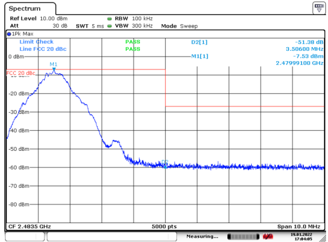
Figure 8.6-5: Band edge spurious emissions at 2483.5 MHz
