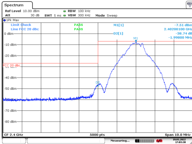
Figure 8.6-4: Band edge spurious emissions at 2400 MHz
