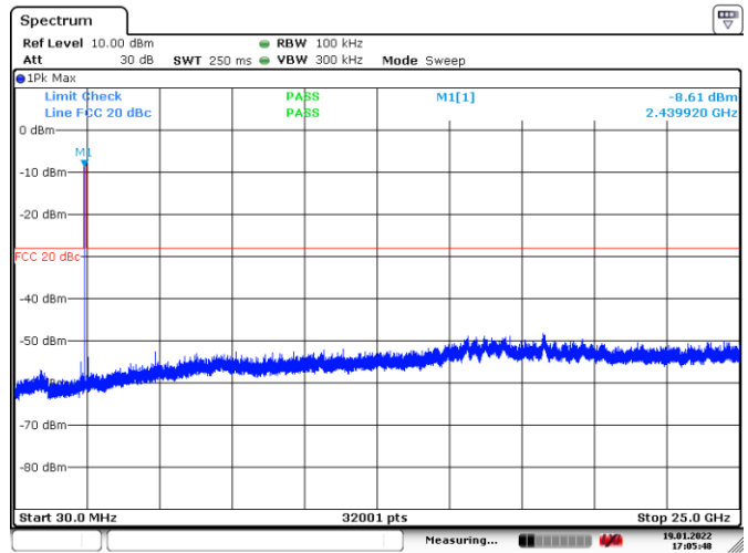
Figure 8.6-2: Conducted spurious emissions Tx on mid channel
