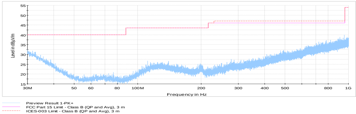
Figure 8.6-7: Radiated spurious emissions 30 MHz to 1GHz, Tx at low channel
