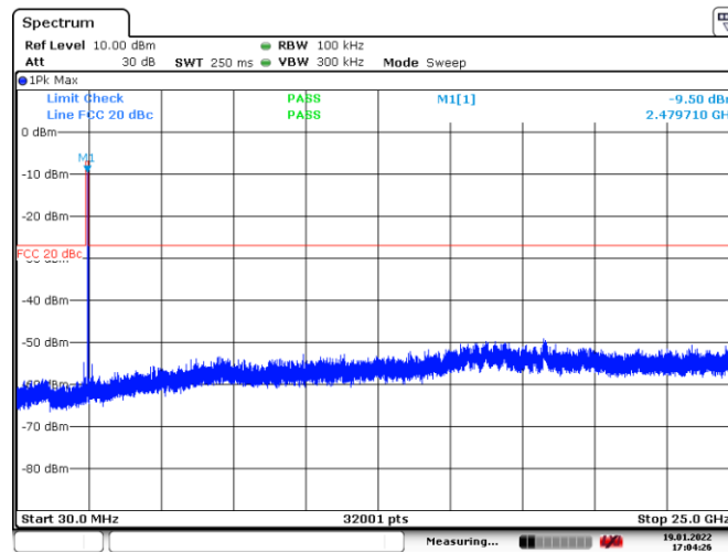
Figure 8.6-3: Conducted spurious emissions Tx on high channel
