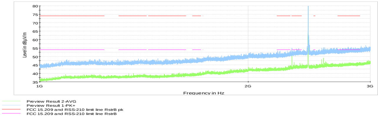
Figure 8.6-10: Radiated spurious emissions 1 to 3GHz, Tx at low channel
