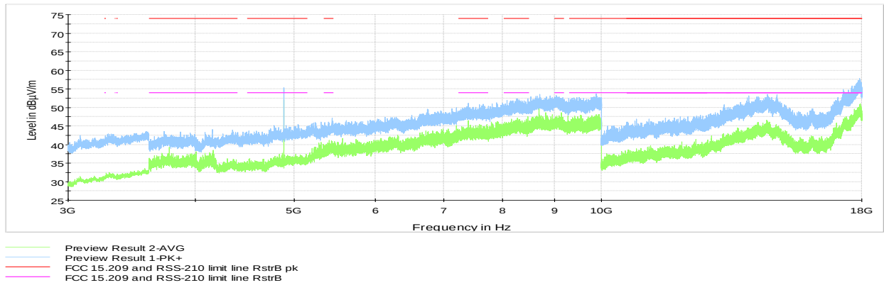
Figure 8.6-13: Radiated spurious emissions 3 to 18GHz, Tx at low channel
