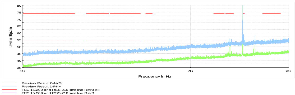
Figure 8.6-11: Radiated spurious emissions 1 to 3GHz, Tx at low channel
