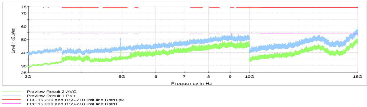
Figure 8.6-14: Radiated spurious emissions 3 to 18GHz, Tx at low channel
