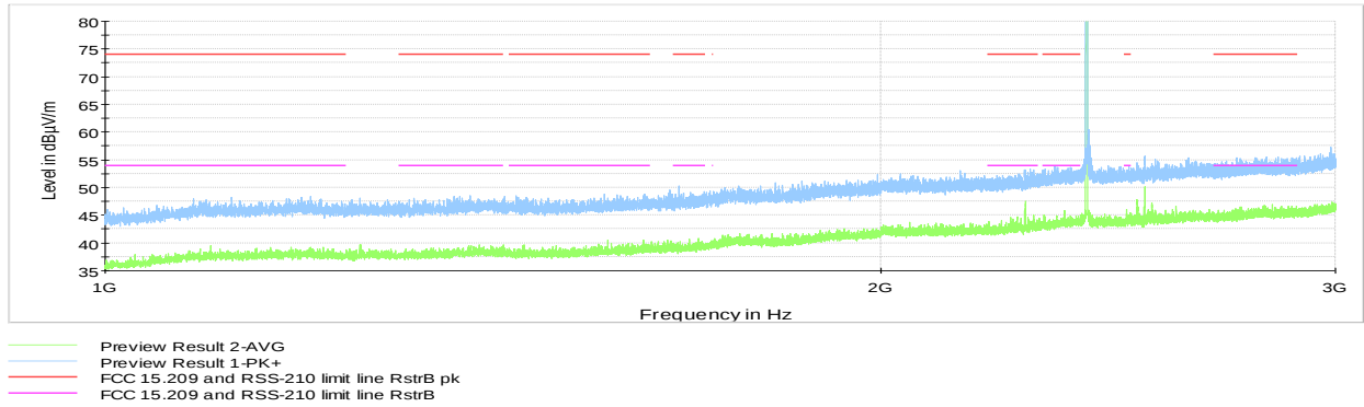
Figure 8.6-9: Radiated spurious emissions 1 to 3GHz, Tx at low channel
