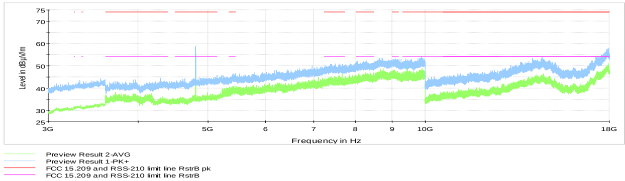
Figure 8.6-12: Radiated spurious emissions 3 to 18GHz, Tx at low channel
