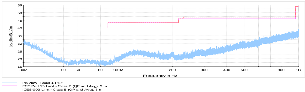
Figure 8.6-8: Radiated spurious emissions 30 MHz to 1GHz, Tx at low channel
