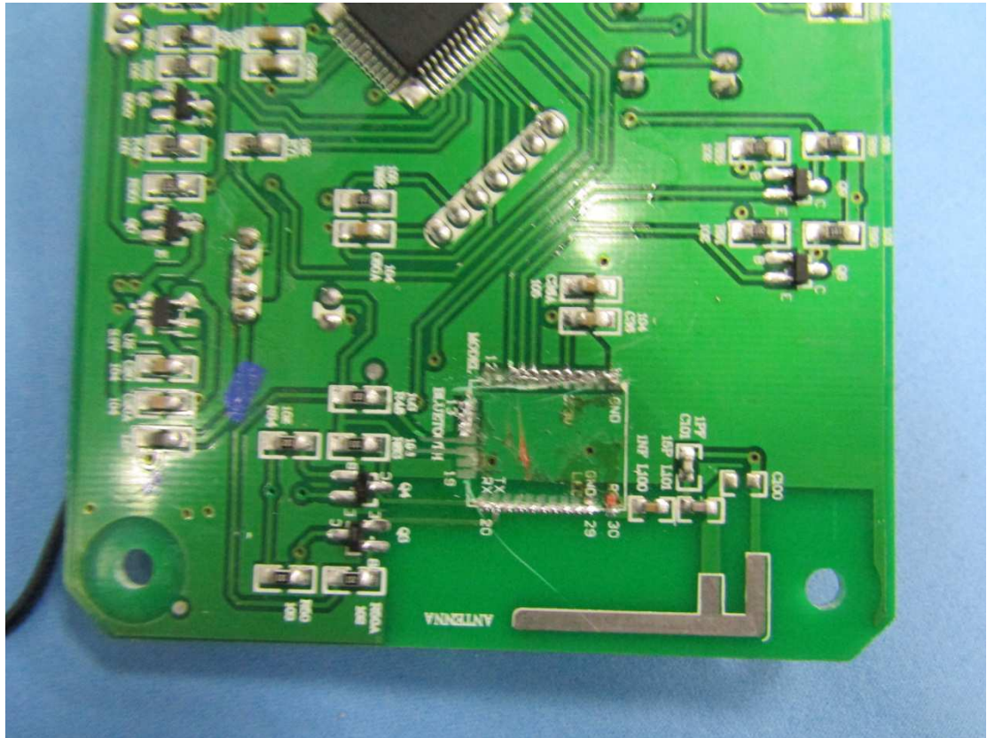
Control PCB view (Remove Bluetooth module view )
