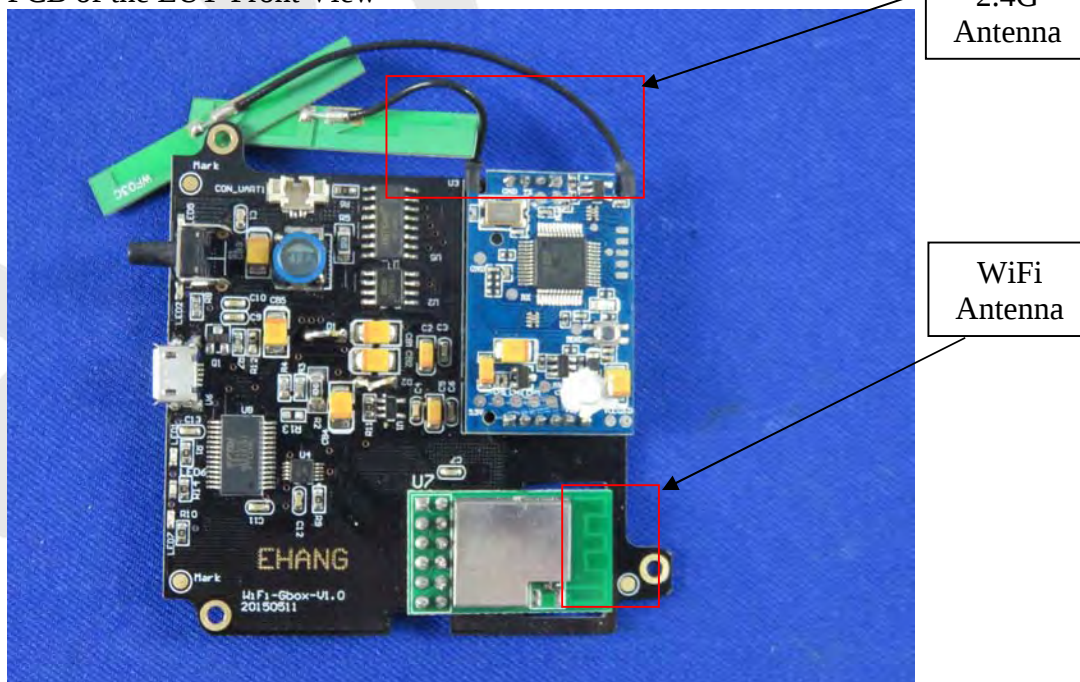
Figure 9 PCB of the EUT-Front View
