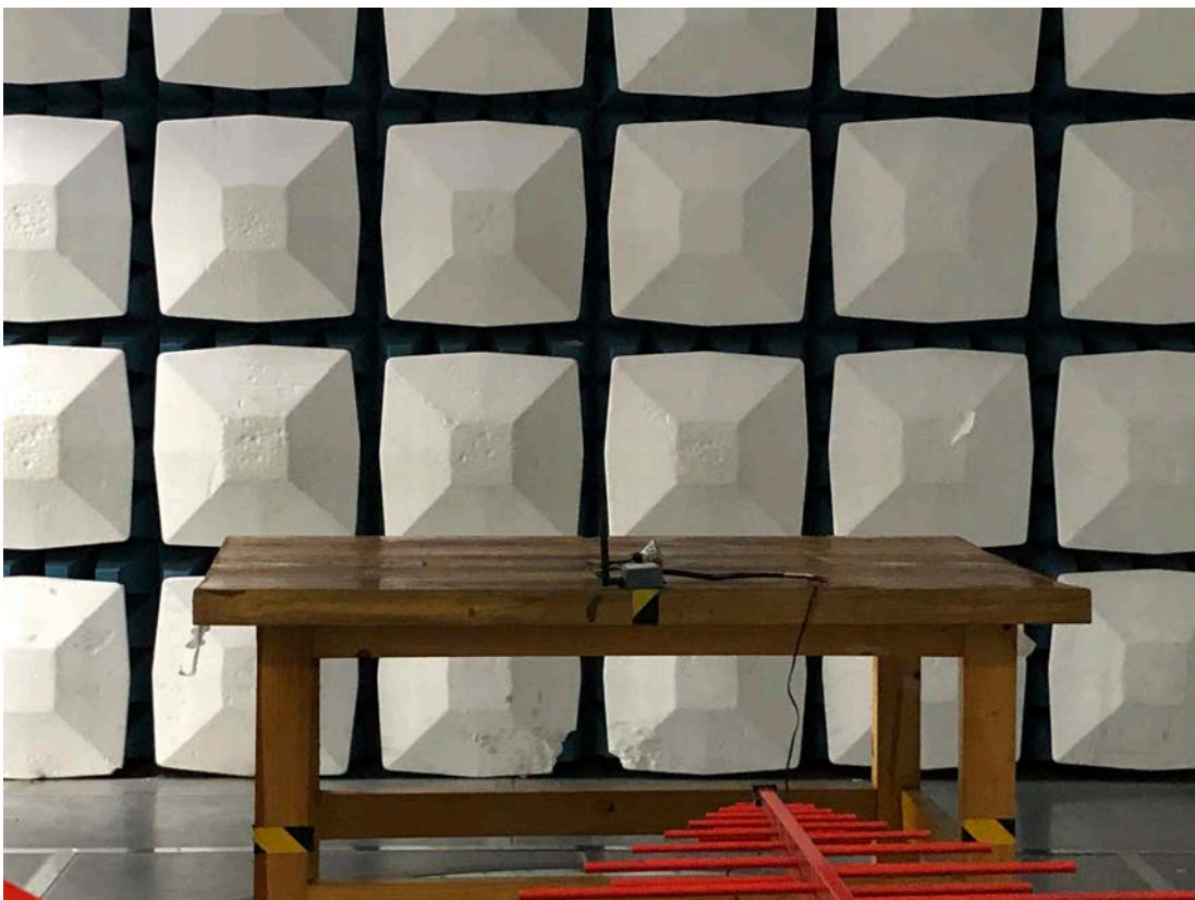
Radiated Emission Below 1GHz Back View
