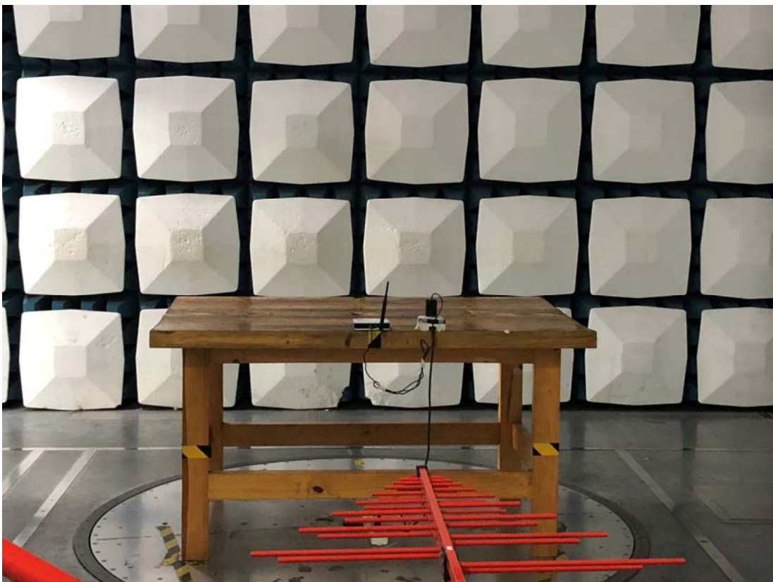
Radiated Emission Below 1GHz Side View
