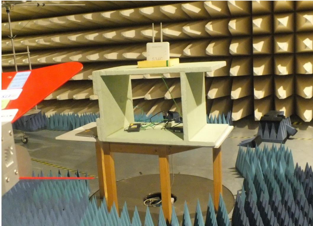
Anechoic chamber
