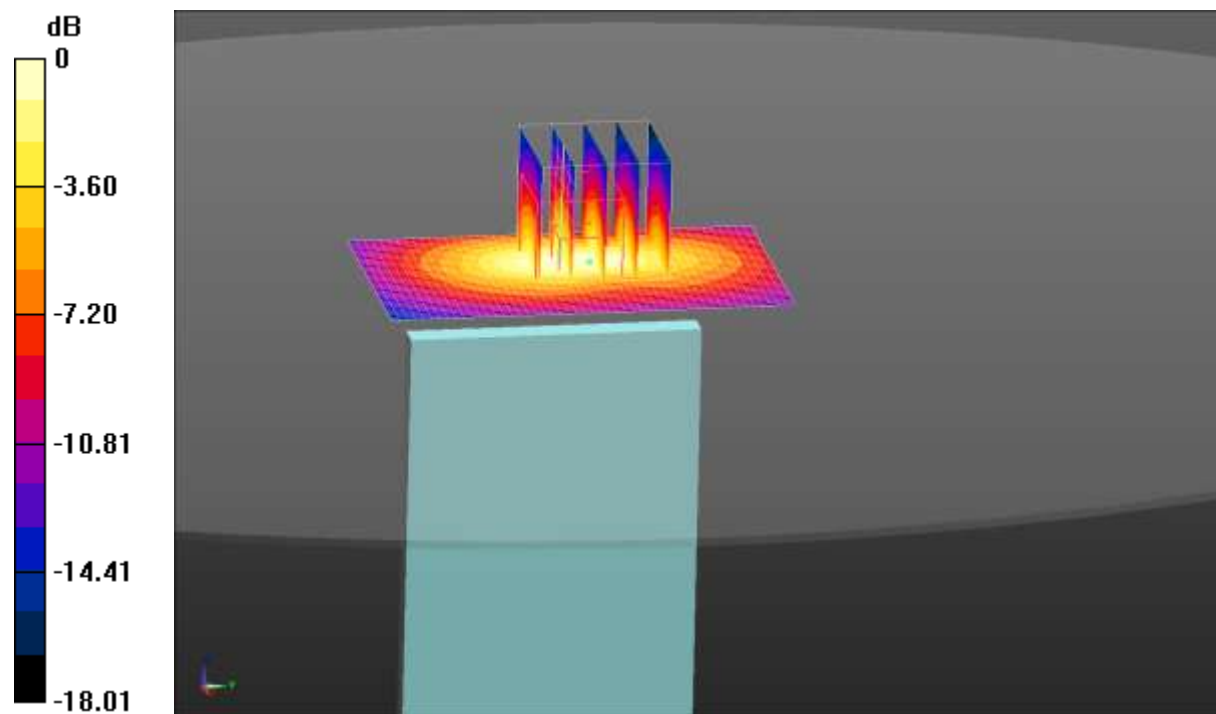
0 dB = 1.45 W/kg = 1.61 dBW/kg
