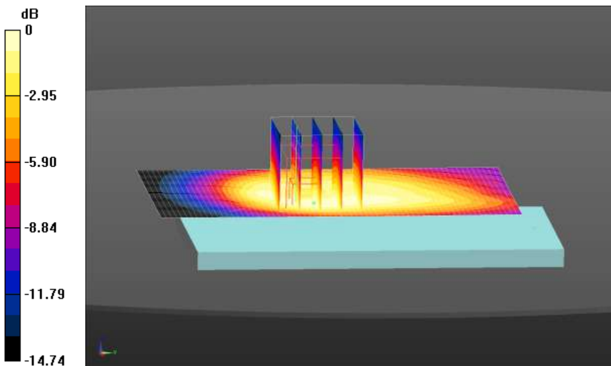
0 dB = 0.573 W/kg = -2.42 dBW/kg
