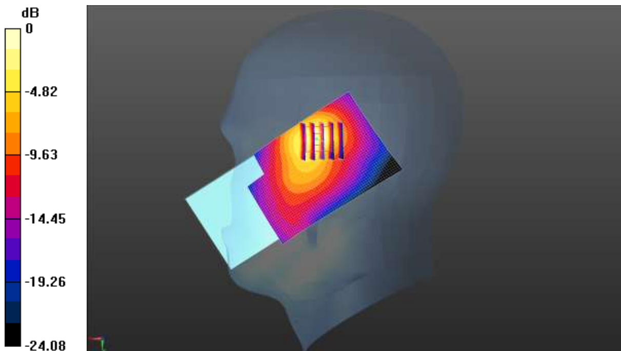
0 dB = 0.309 W/kg = -5.10 dBW/kg
