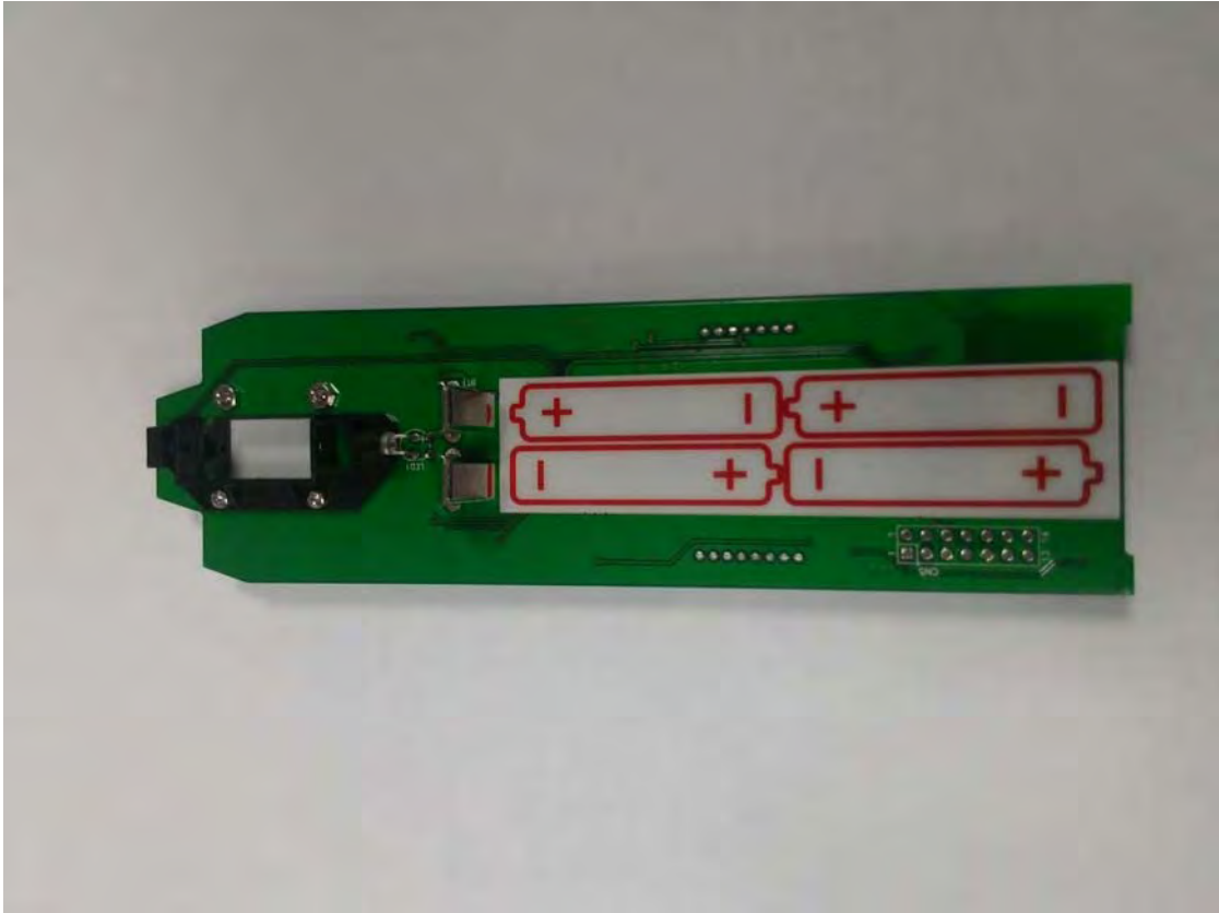
09 Rear view of PCB
