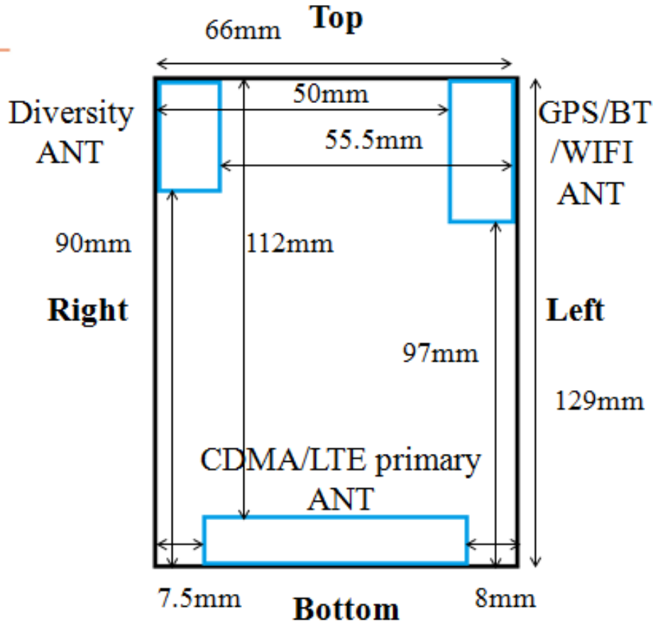
Fig.17 Antenna position of EUT (Back View)
