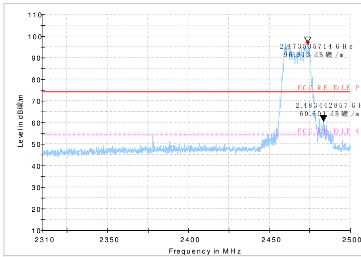
Fig.69 Radiated emission (Power): 802.11g, channel 12
