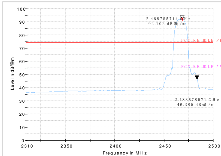
Fig.86 Radiated emission (Power): 802.11g, channel12
