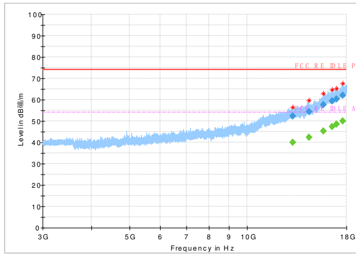
Fig.59 Radiated Spurious Emission (802.11b,Ch11,3GHz~18GHz)
