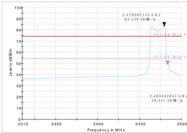
Fig.81 Radiated emission (Power): 802.11n, channel 13
