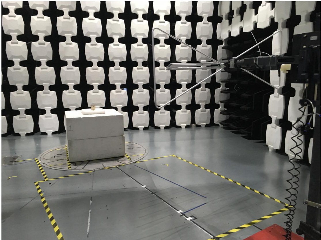
Description: Radiated Emission Test Setup (30-1000MHz)
