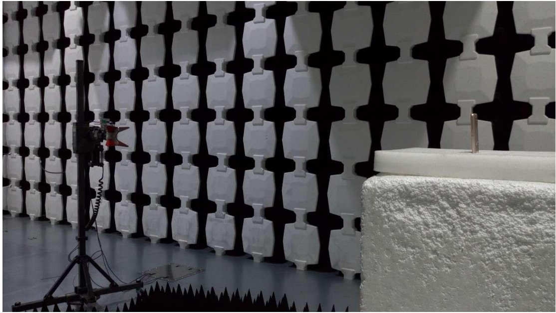
Description: Radiated Emission Test Setup (1-18GHz)
