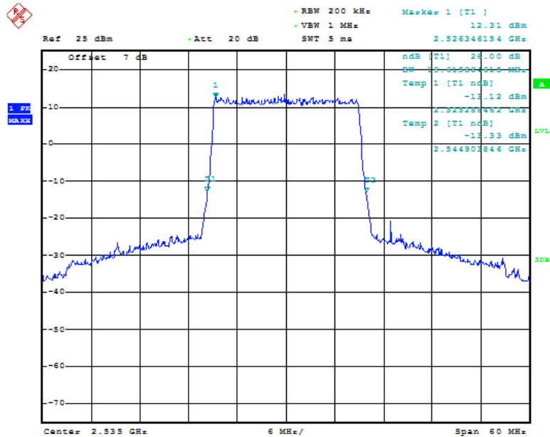
Fig.79 LTE band 7, 20MHz Bandwidth, QPSK (-26dBc BW)
