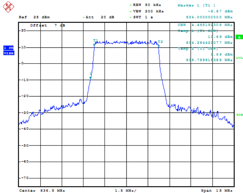
Fig.29 LTE band 5, 5MHz Bandwidth, QPSK (99% BW)
