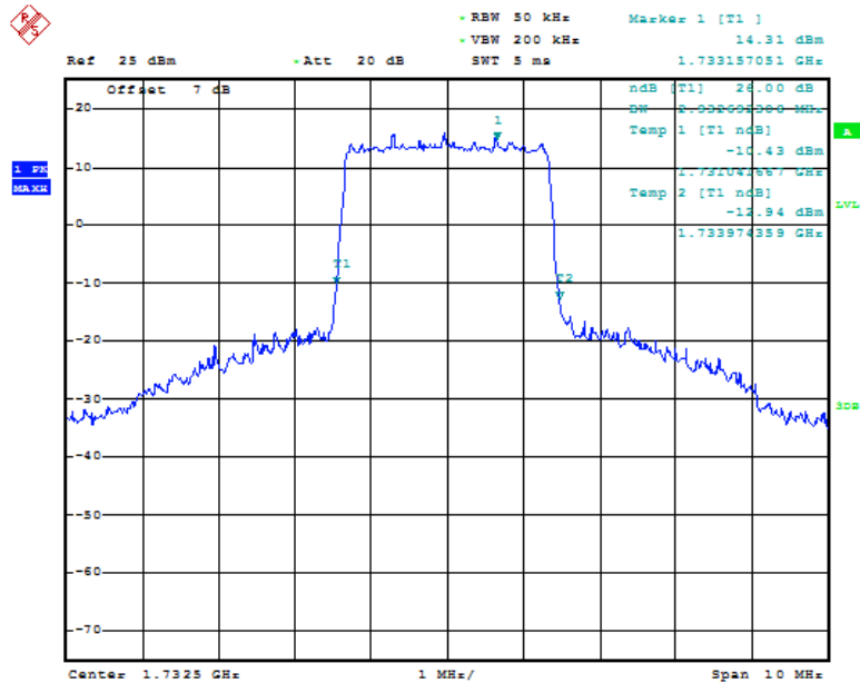
Fig.55 LTE band 4, 3MHz Bandwidth, QPSK (-26dBc BW)
