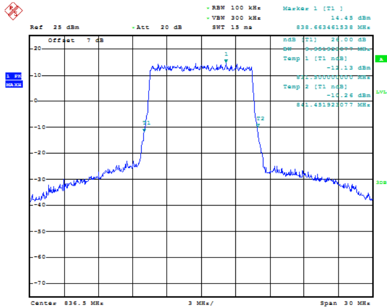
Fig.71 LTE band 5, 10MHz Bandwidth, QPSK (-26dBc BW)
