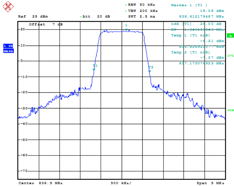
Fig.65 LTE band 5, 1.4MHz Bandwidth, QPSK (-26dBc BW)
