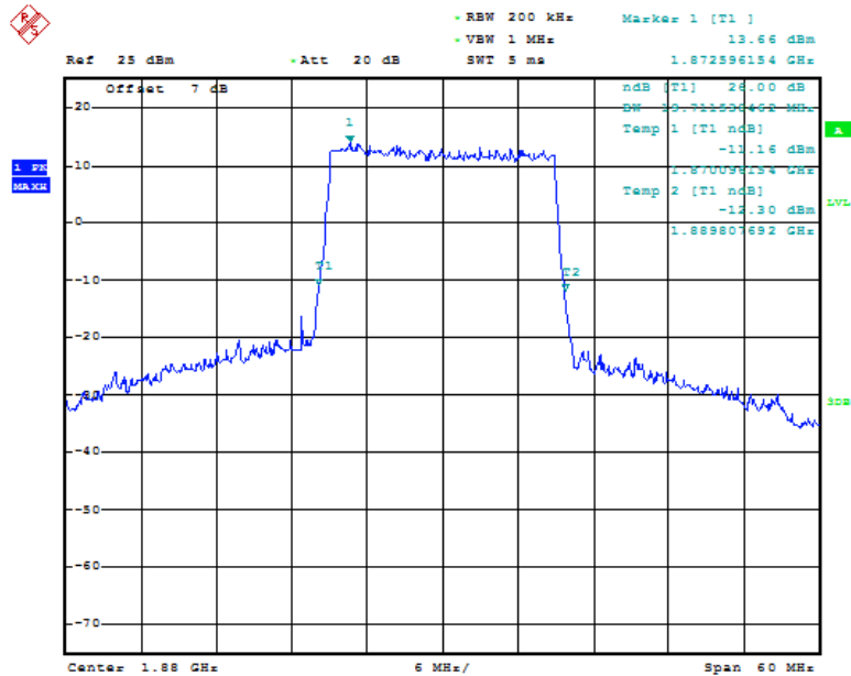
Fig.51 LTE band 2, 20MHz Bandwidth, QPSK (-26dBc BW)
