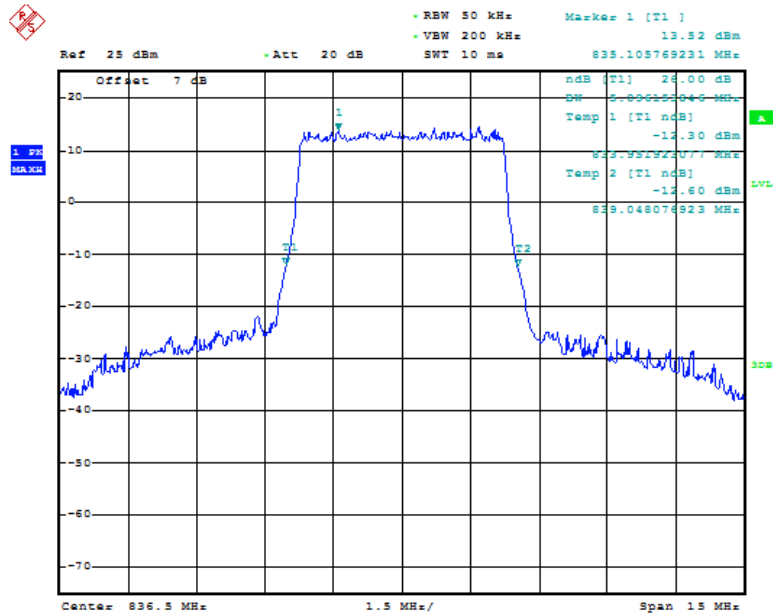
Fig.69 LTE band 5, 5MHz Bandwidth, QPSK (-26dBc BW)
