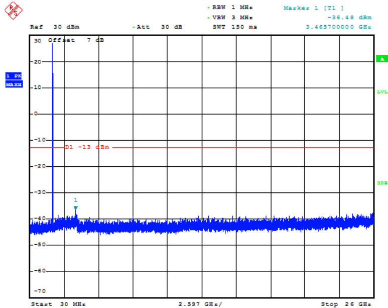
Fig.97 LTE band 2: 30MHz – 26GHz
