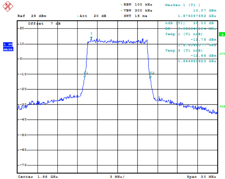
Fig.47 LTE band 2, 10MHz Bandwidth, QPSK (-26dBc BW)
