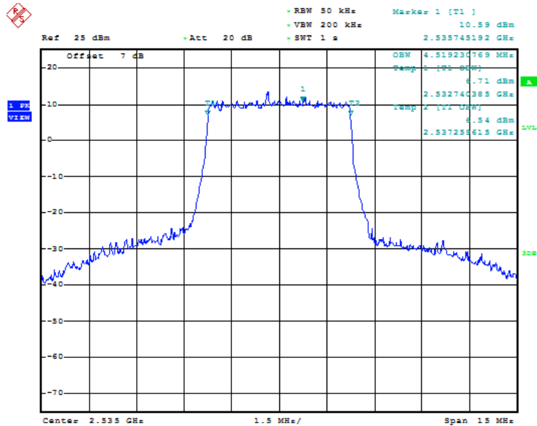
Fig.33 LTE band 7, 5MHz Bandwidth, QPSK (99% BW)
