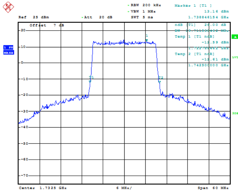
Fig.63 LTE band 4, 20MHz Bandwidth, QPSK (-26dBc BW)
