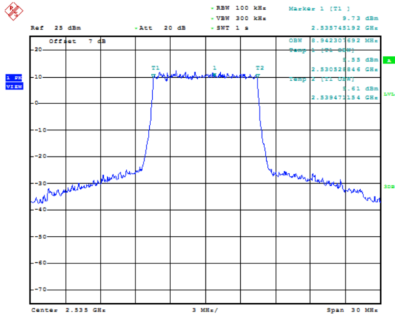
Fig.35 LTE band 7, 10MHz Bandwidth, QPSK (99% BW)
