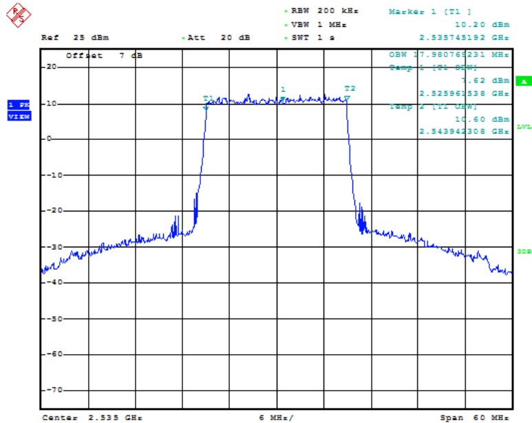
Fig.39 LTE band 7, 20MHz Bandwidth, QPSK (99% BW)
