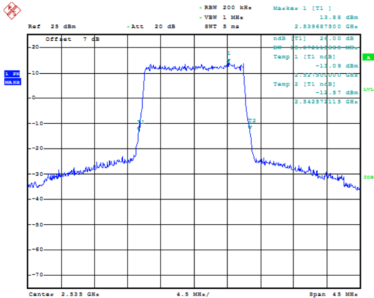
Fig.77 LTE band 7, 15MHz Bandwidth, QPSK (-26dBc BW)
