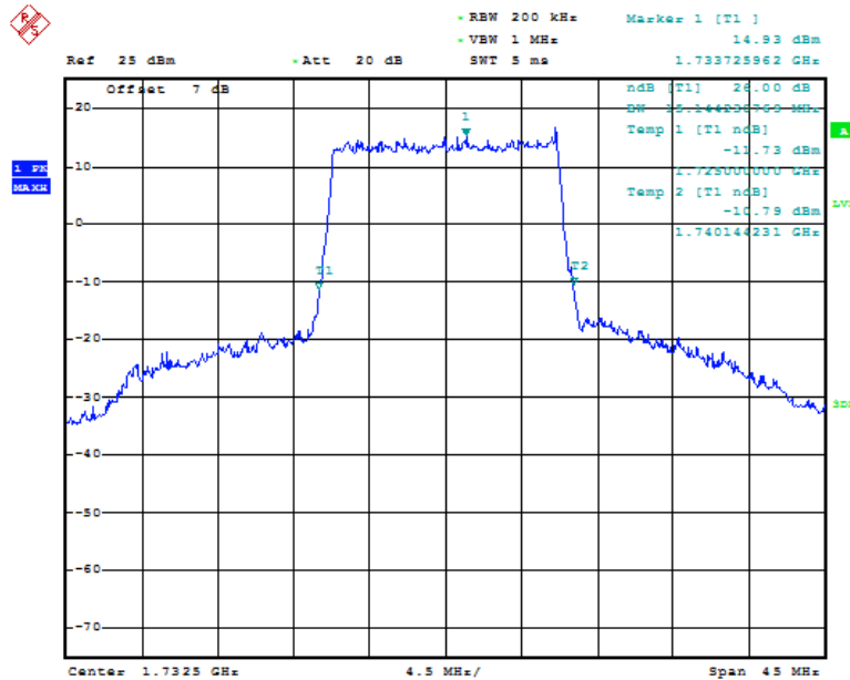
Fig.61 LTE band 4, 15MHz Bandwidth, QPSK (-26dBc BW)
