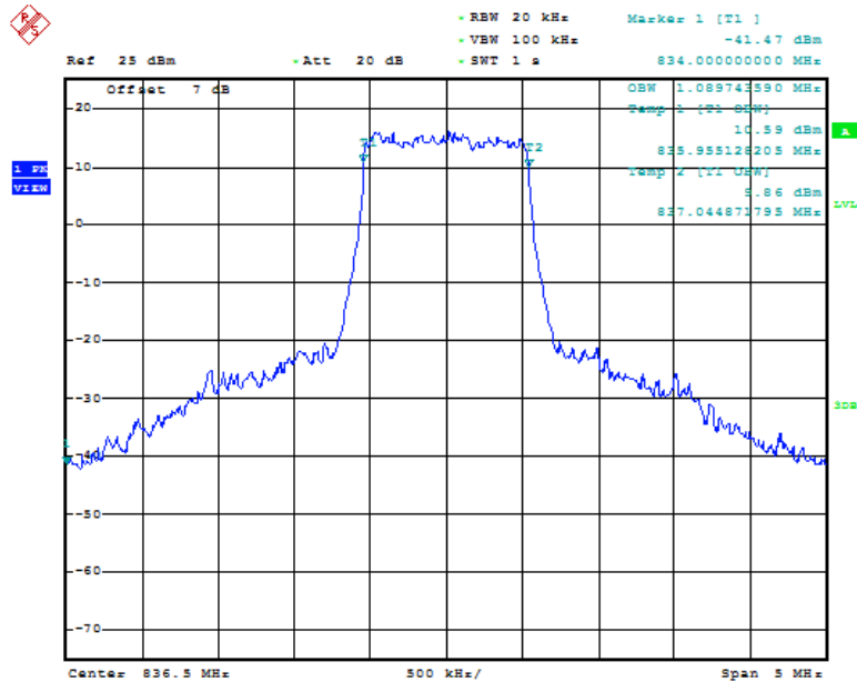
Fig.25 LTE band 5, 1.4MHz Bandwidth, QPSK (99% BW)
