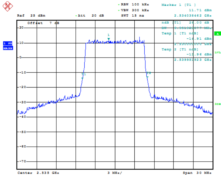
Fig.75 LTE band 7, 10MHz Bandwidth, QPSK (-26dBc BW)
