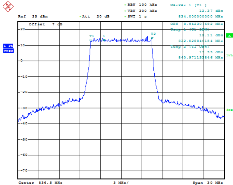
Fig.31 LTE band 5, 10MHz Bandwidth, QPSK (99% BW)
