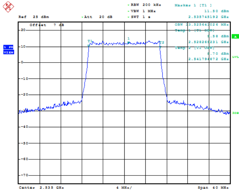
Fig.37 LTE band 7, 15MHz Bandwidth, QPSK (99% BW)
