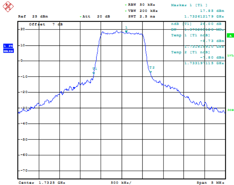
Fig.53 LTE band 4, 1.4MHz Bandwidth, QPSK (-26dBc BW)
