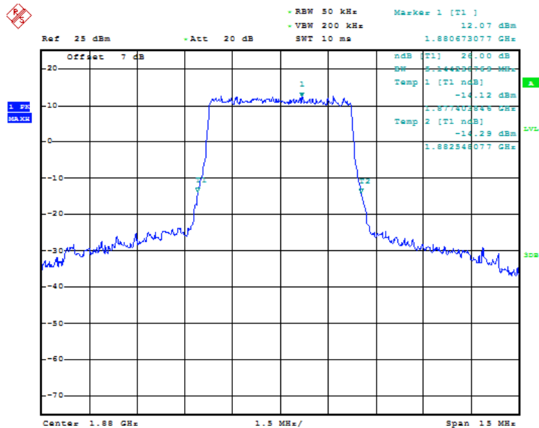
Fig.45 LTE band 2, 5MHz Bandwidth, QPSK (-26dBc BW)
