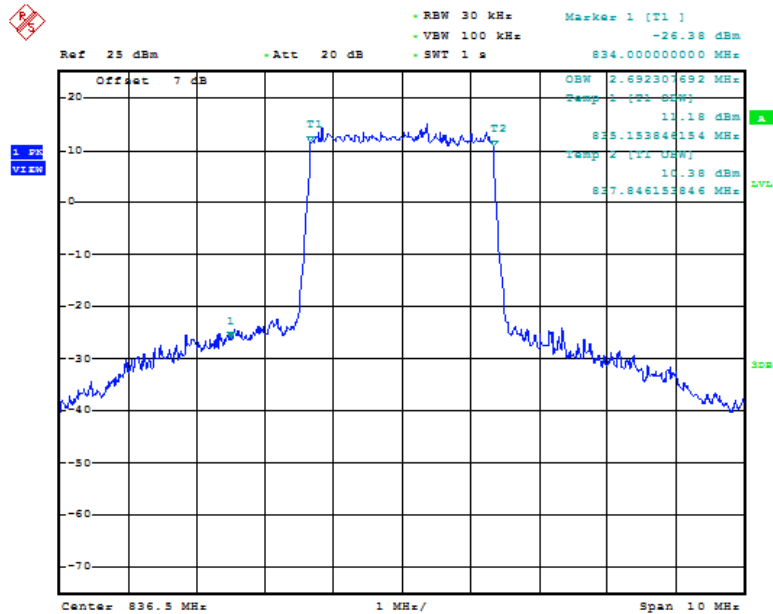
Fig.27 LTE band 5, 3MHz Bandwidth, QPSK (99% BW)
