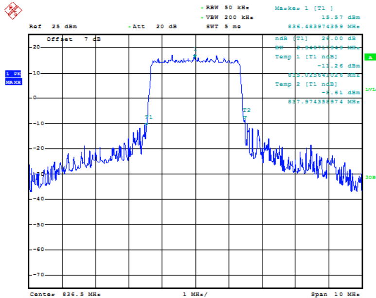
Fig.67 LTE band 5, 3MHz Bandwidth, QPSK (-26dBc BW)
