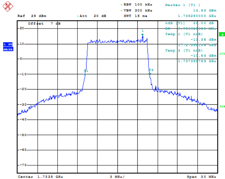
Fig.59 LTE band 4, 10MHz Bandwidth, QPSK (-26dBc BW)
