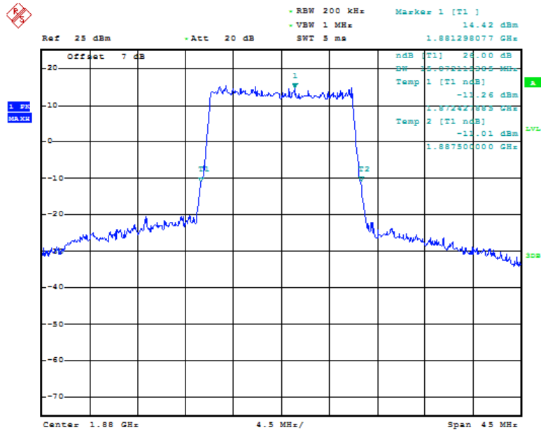
Fig.49 LTE band 2, 15MHz Bandwidth, QPSK (-26dBc BW)
