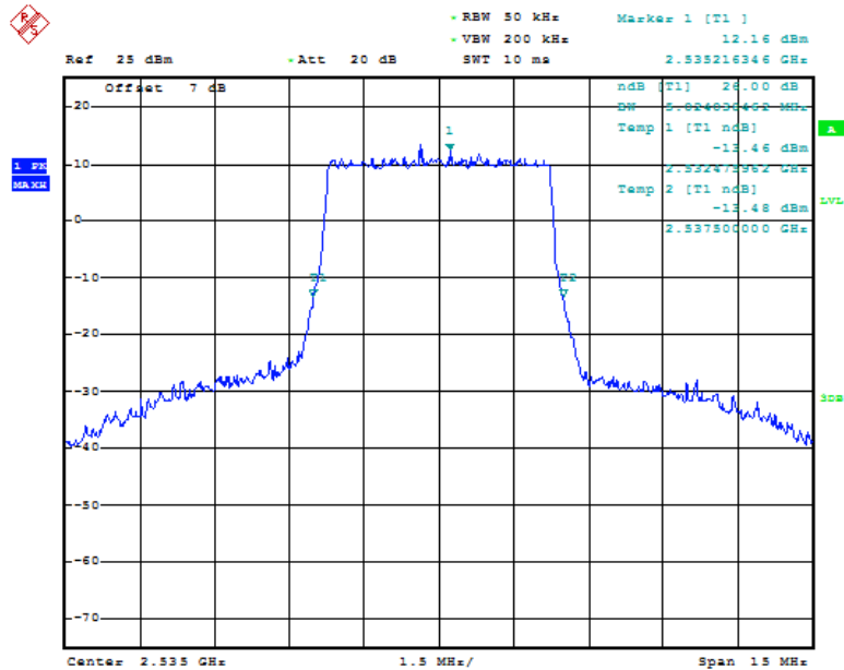
Fig.73 LTE band 7, 5MHz Bandwidth, QPSK (-26dBc BW)
