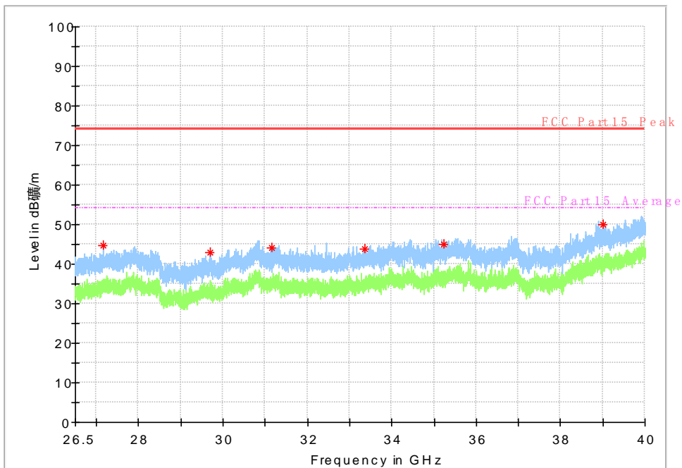
Fig. 28 Radiated emission: 802.11n, (802.11n-HT20, Ch149, 26.5 GHz - 40 GHz)
