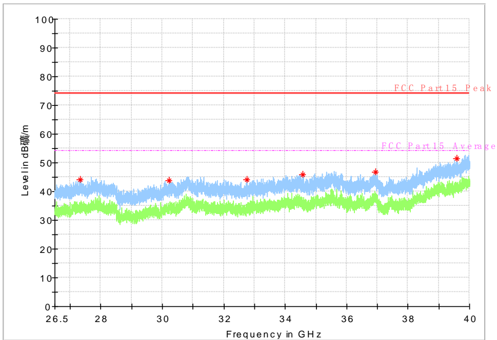
Fig. 23 Radiated emission: 802.11n, (802.11a, Ch149, 26.5 GHz - 40 GHz)
