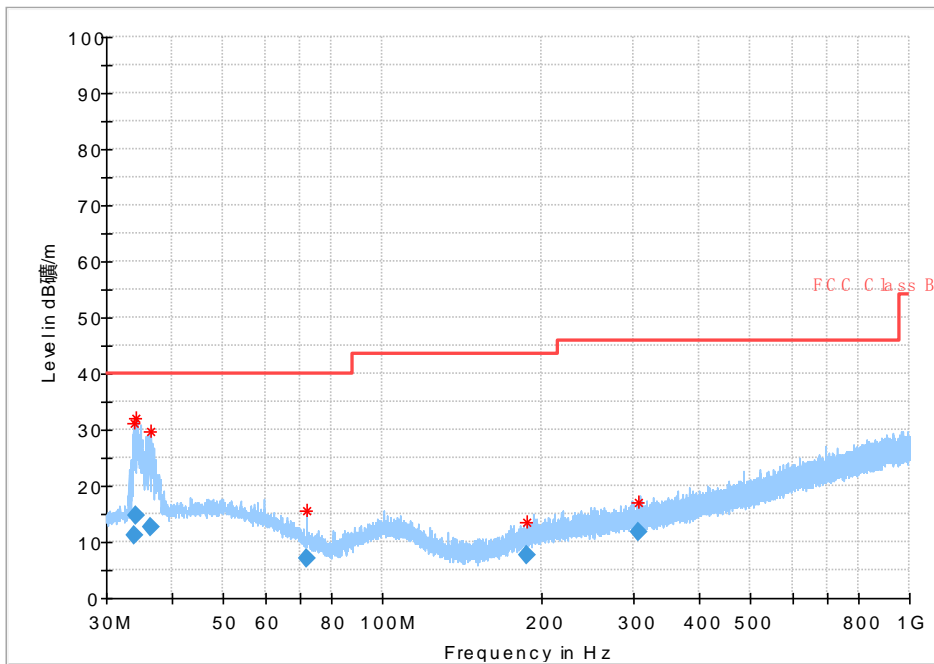
Fig. 29 Radiated Spurious Emission (802.11a, Ch149, 30 MHz-1 GHz)
