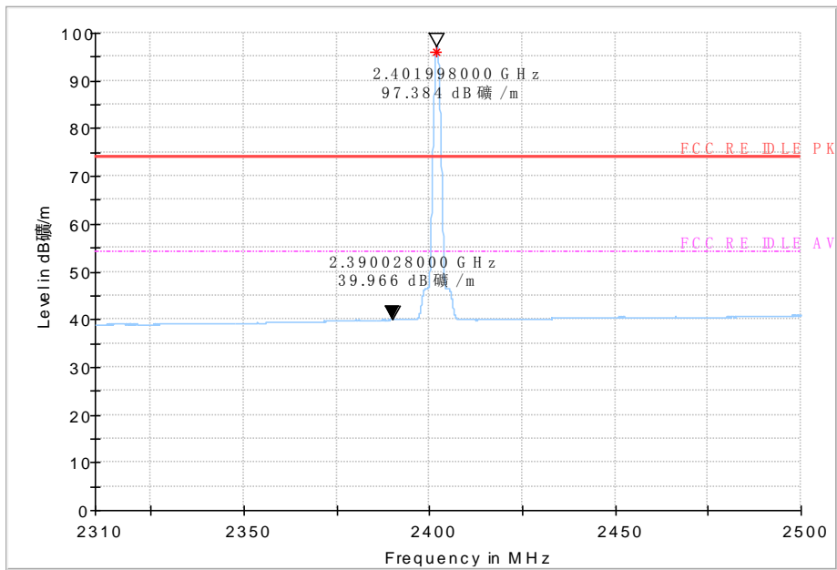
Fig.21 Bandedge: CH0
