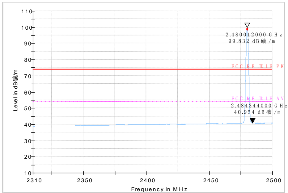
Fig.25 Bandedge:CH39
