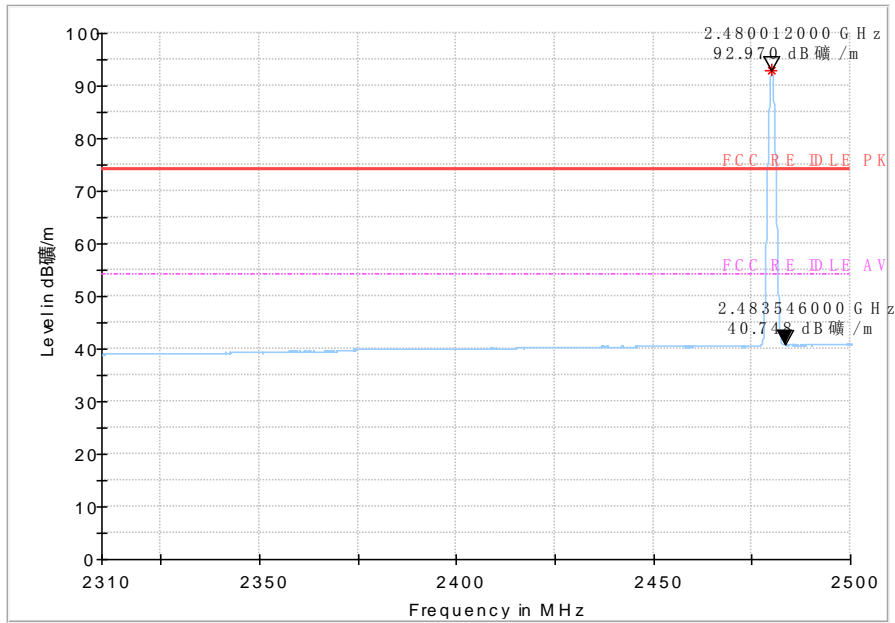
Fig.29 Bandedge:CH39
