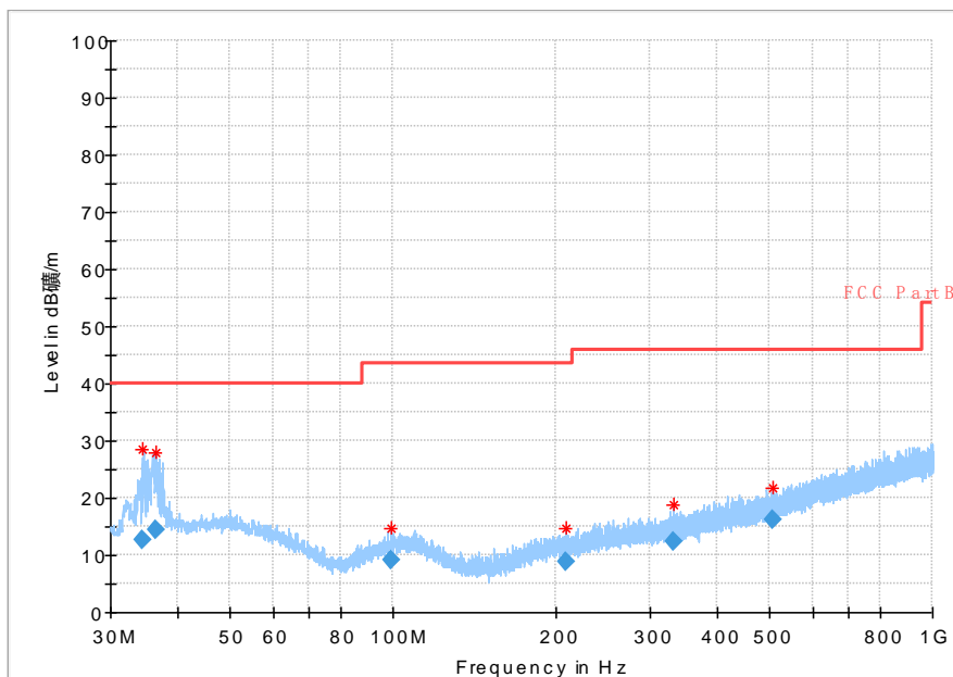
Fig.26 Radiated emission: CH39, 30MHz~1GHz
