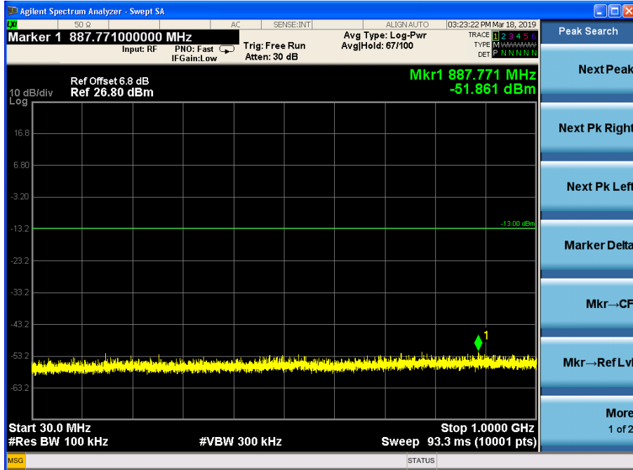
Channel 9400, 30MHz~1GHz
