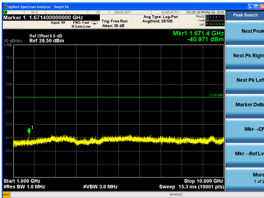
Channel 4183, 1GHz~10GHz
