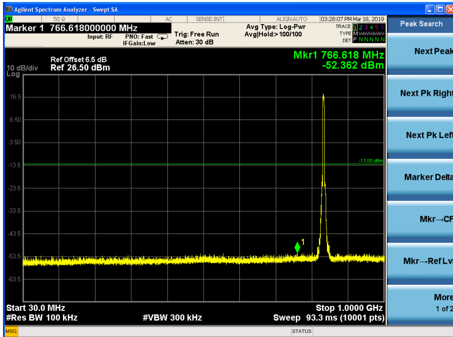
Channel 4183, 30MHz~1GHz
