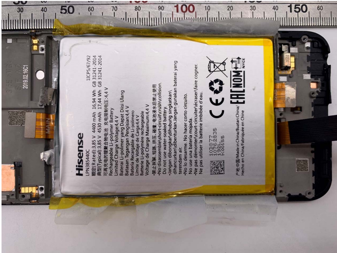
Battery View 2 (LPN385440C made by Ningbo Veken Battery Co. Ltd.)
