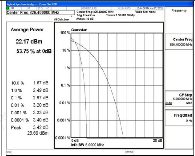
Channel 4132 / 826.4 MHz
