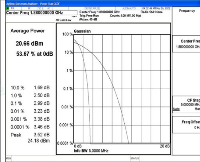
Channel 9400 / 1880.0 MHz
