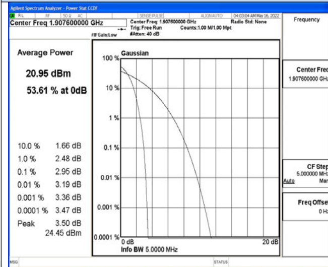
Channel 9538 / 1907.6 MHz
