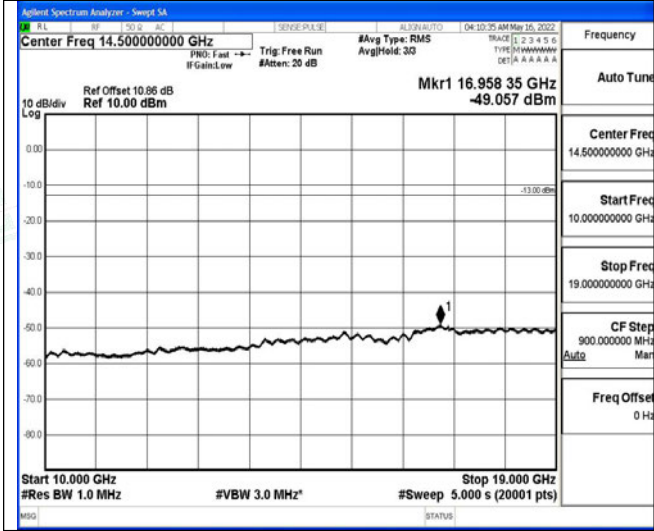
10 GHz – 19 GHz
