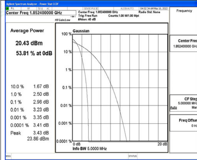
Channel 9262 / 1852.4 MHz
