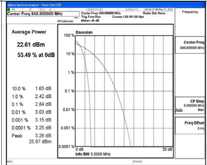
Channel 4233 / 846.6 MHz
