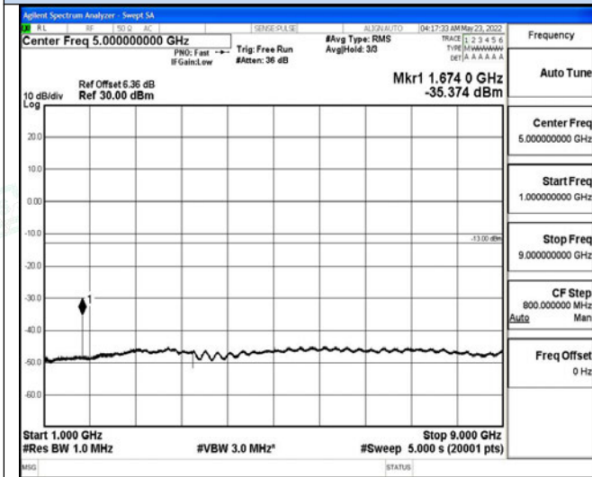
1 GHz – 9 GHz
