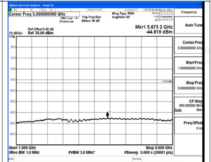
1 GHz – 9 GHz
