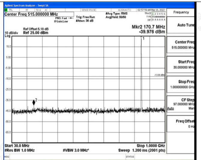
30 MHz – 1000 MHz
