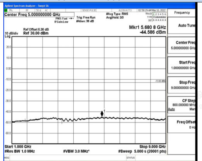
1 GHz – 9 GHz
