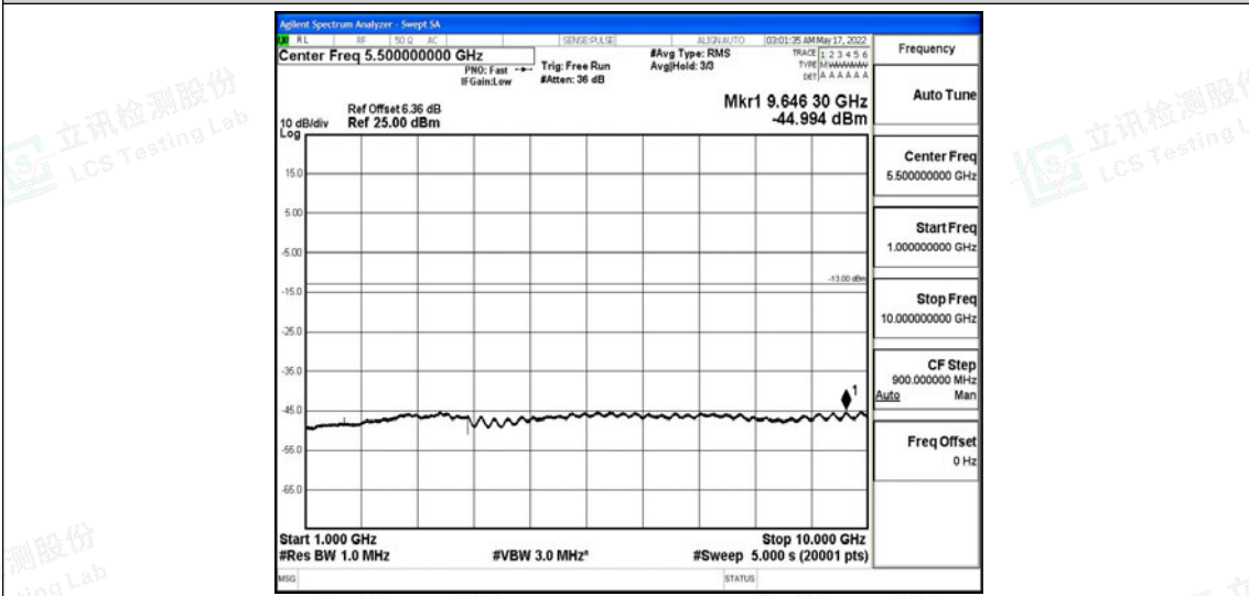
Band26-10MHz-16QAM-26740-1RB#0-Range4:1000~10000MHz
