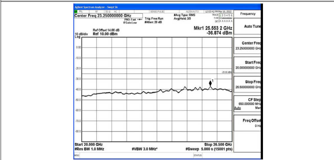
Band7-20MHz-16QAM-21350-1RB#0-Range6:20000~26500MHz
