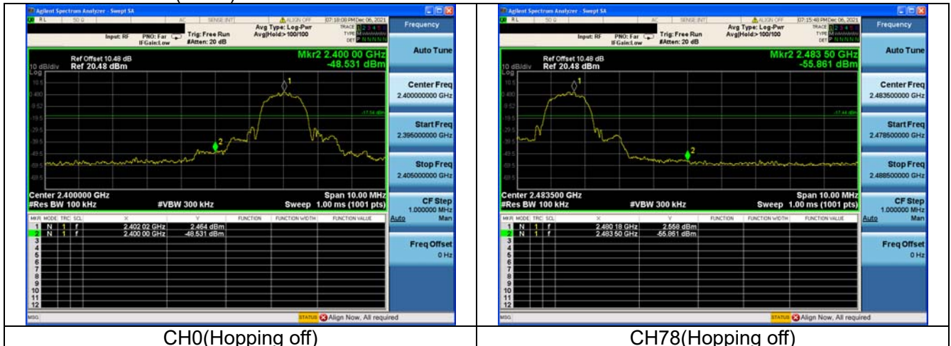
CH0(Hopping off)
