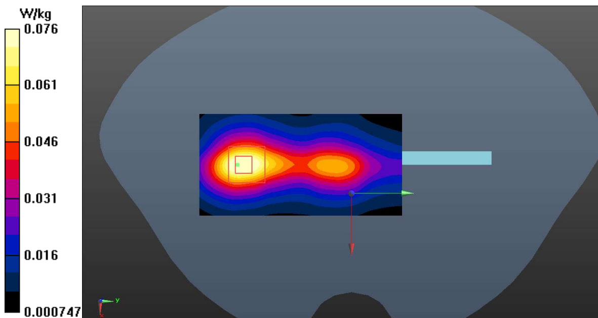
Fig.26 WLAN 2.4GHz Body
