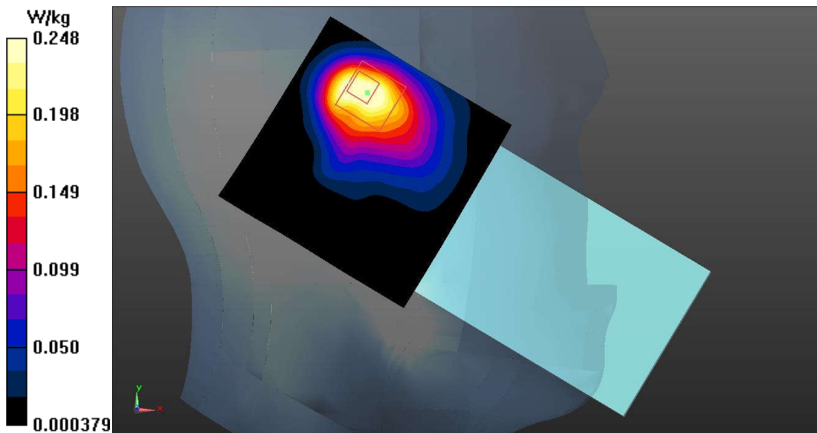
Fig.25 WLAN 2.4GHz Head
