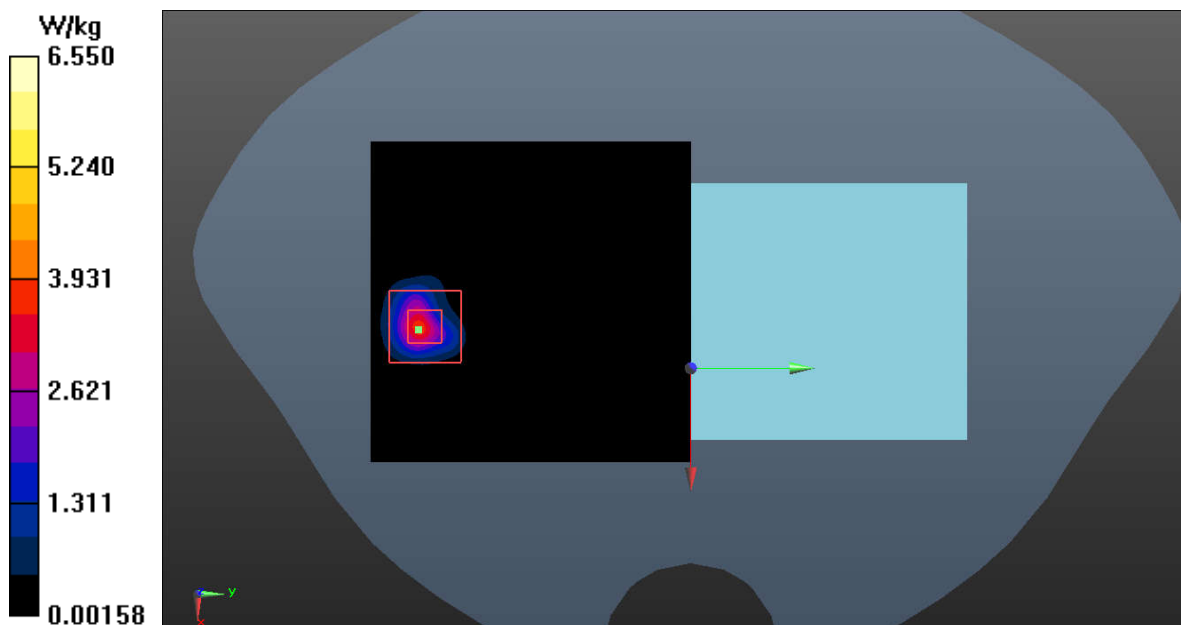
Fig.29 WLAN 5GHz Extremity
