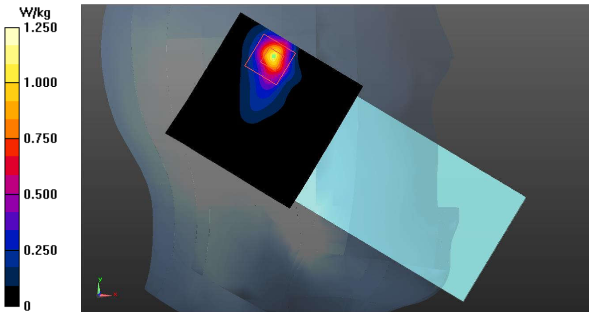
Fig.27 WLAN 5GHz Head
