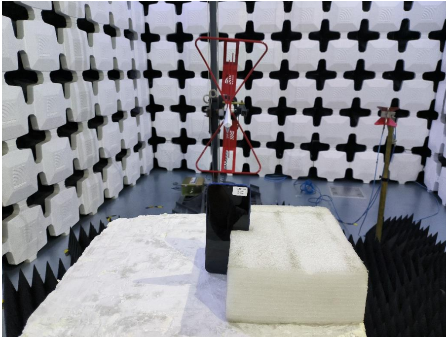
11. Radiated Emissions (Part 15C, 1GHz -18GHz)
