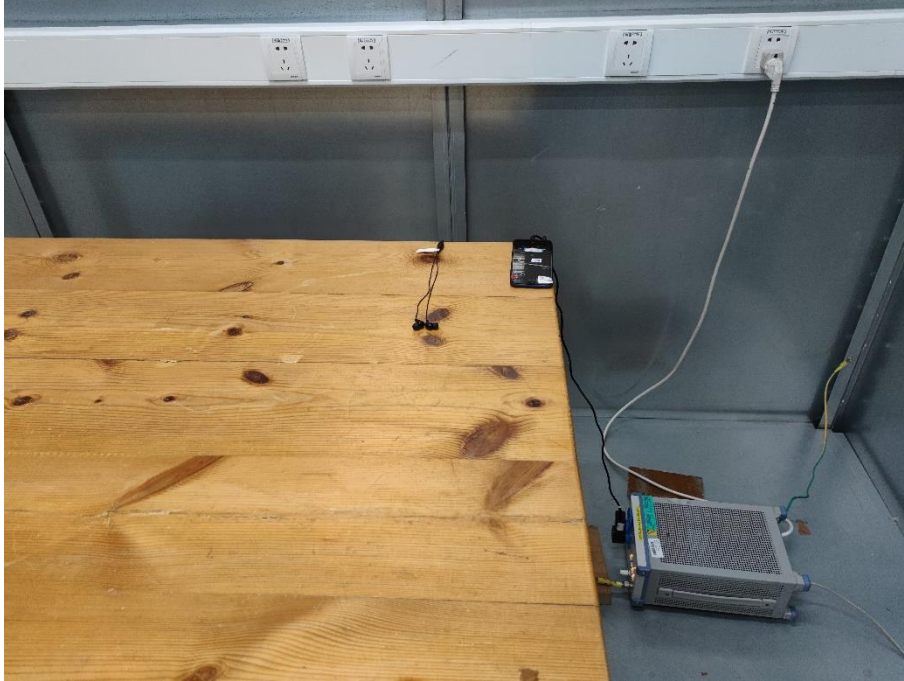
17. Conducted Emission (Part 15B, Camera/Video Player/FM receive)
