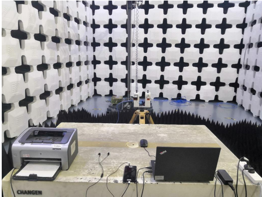
3. Radiated Emissions (Part 15B Data Transfer ,5,18GHz-26.5GHz)
