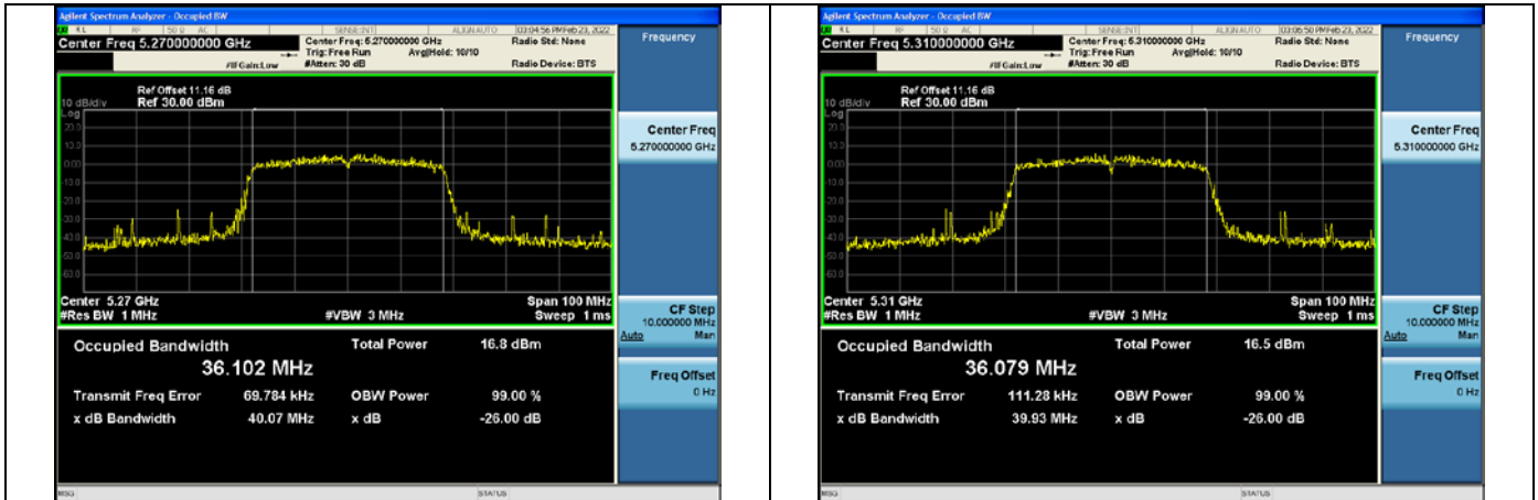
Test Mode:802.11n HT40 5270MHz Chain0
