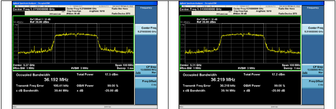
Test Mode:802.11ac VHT40 5270MHz Chain0
