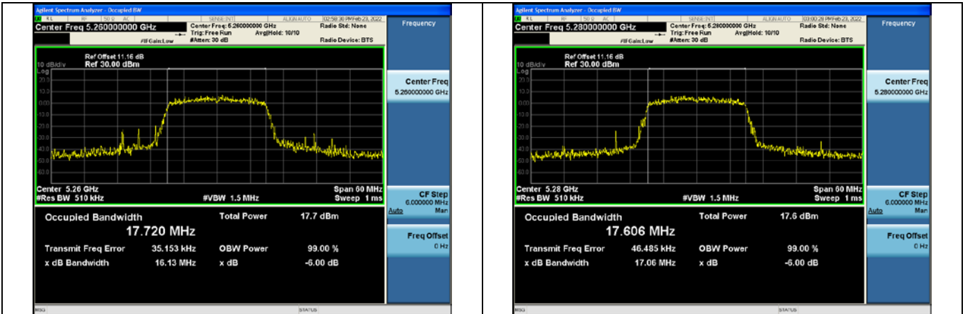
Test Mode:802.11n HT20 5260MHz Chain0
