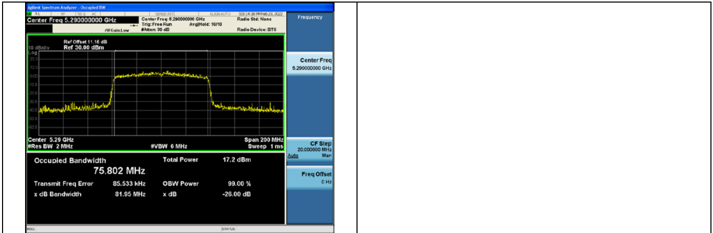
Test Mode:802.11ac VHT80 5290MHz Chain0
