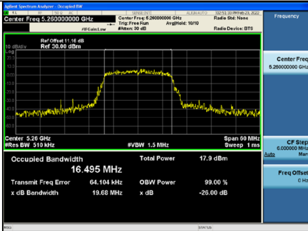
Test Mode:802.11a 5260MHz Chain0
