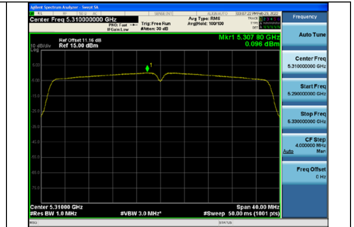
Test Mode:802.11n HT40 5310MHz Chain0
