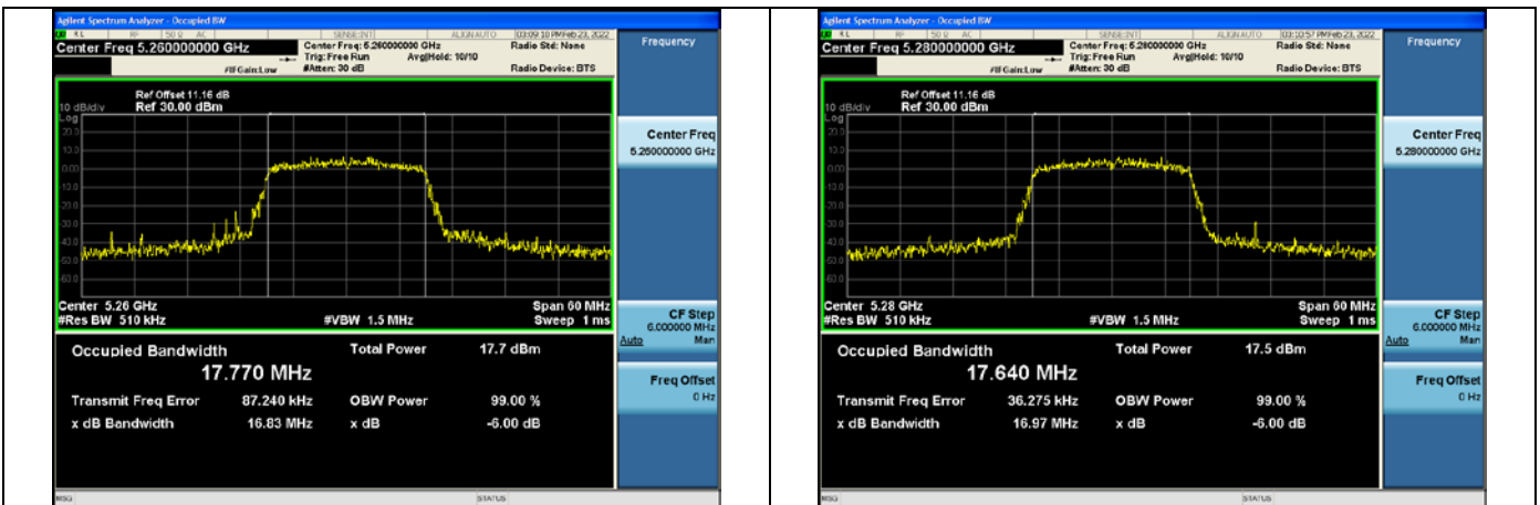
Test Mode:802.11ac VHT20 5260MHz Chain0
