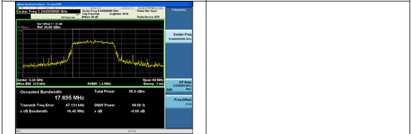
Test Mode:802.11n HT20 5240MHz Chain0
