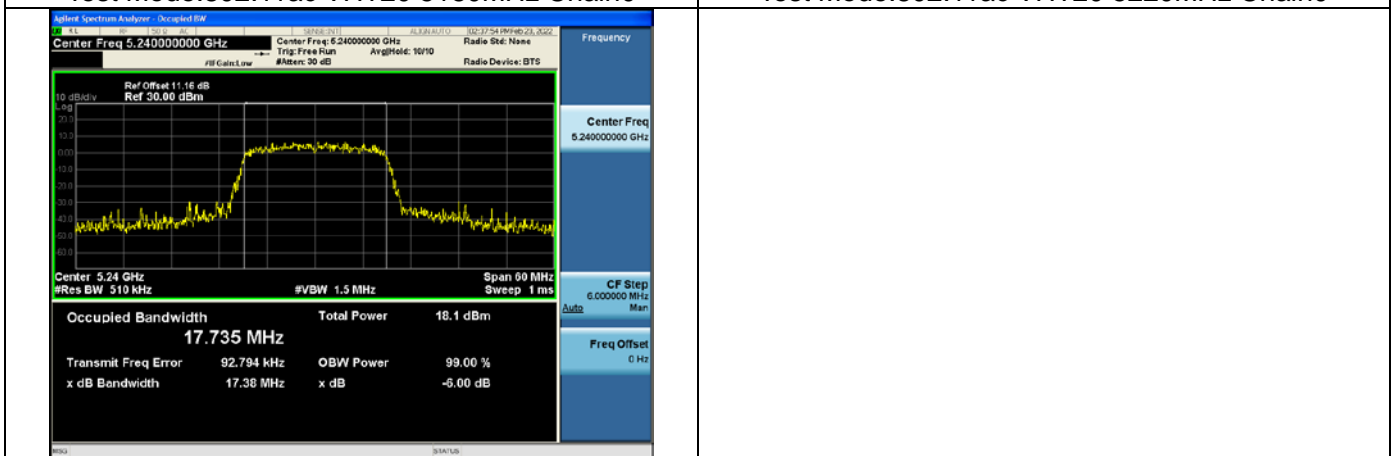
Test Mode:802.11ac VHT20 5240MHz Chain0
