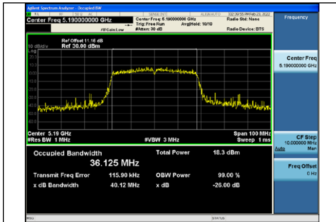
Test Mode:802.11ac VHT40 5190MHz Chain0
