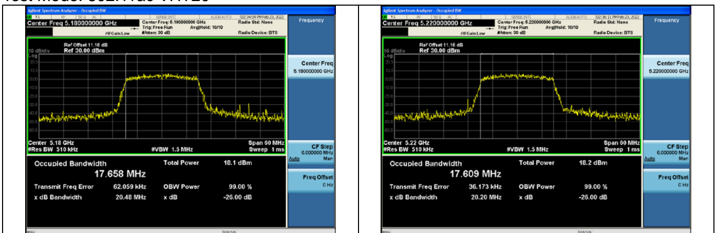
Test Mode:802.11ac VHT20 5180MHz Chain0
