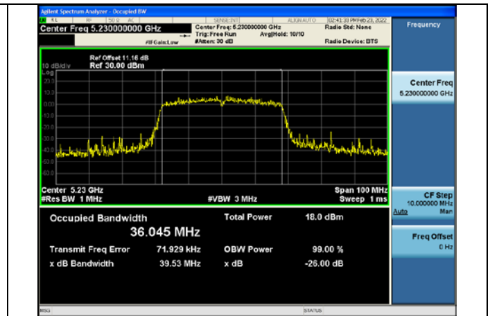
Test Mode:802.11ac VHT40 5230MHz Chain0
