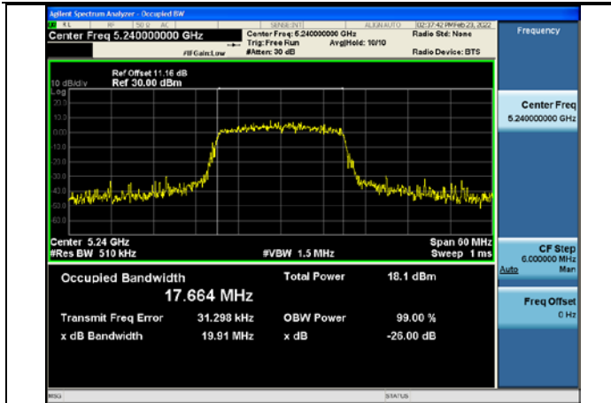
Test Mode:802.11ac VHT20 5240MHz Chain0
