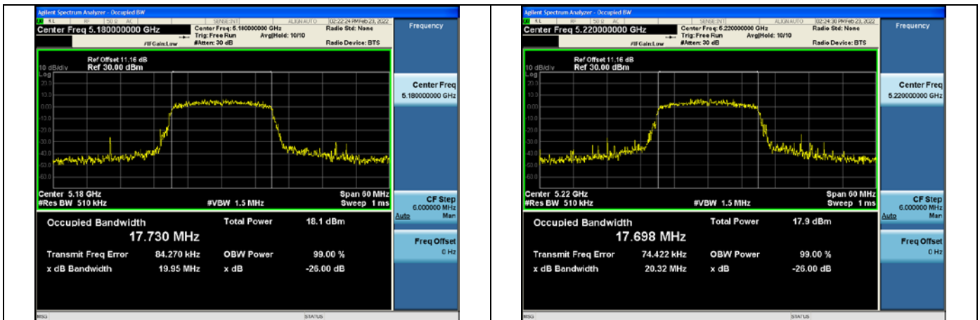
Test Mode:802.11n HT20 5180MHz Chain0
