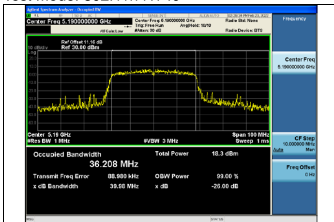
Test Mode:802.11n HT40 5190MHz Chain0
