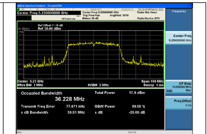
Test Mode:802.11n HT40 5230MHz Chain0
