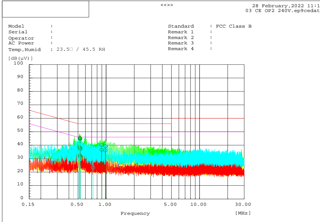
L+N Line
