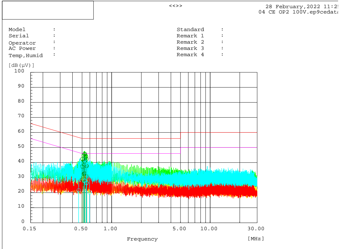
L+N Line
