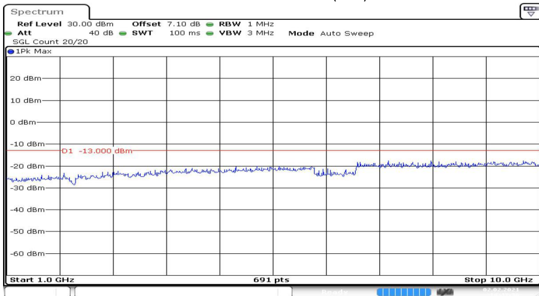
Channel 189 1GHz~10GHz(dBm)
