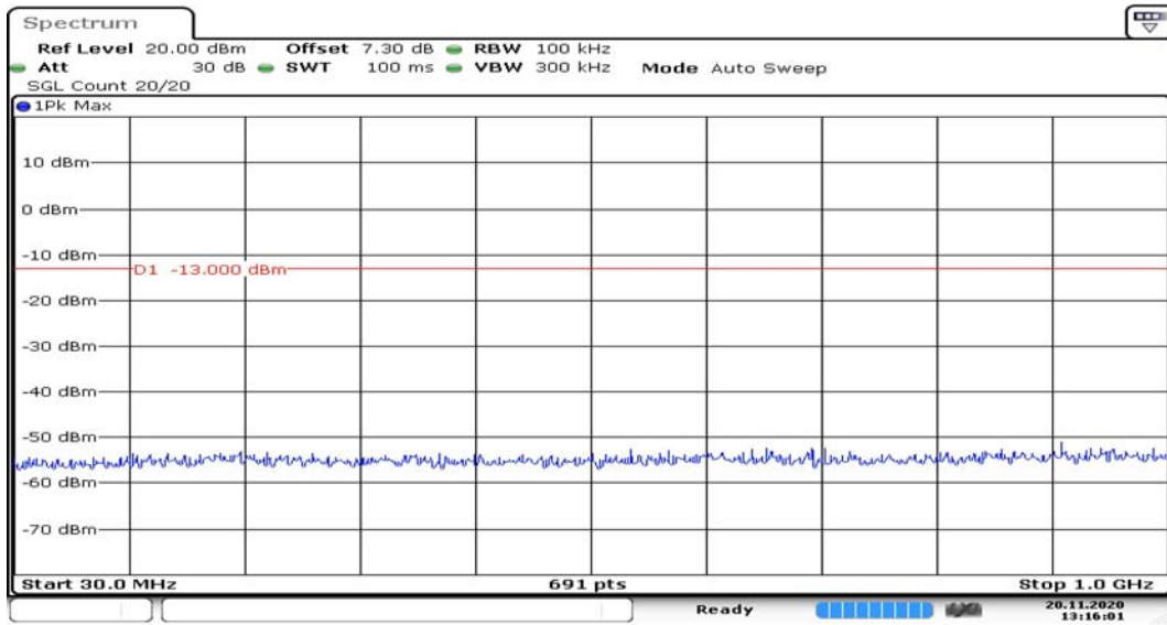
Channel 661 30MHz~1GHz
