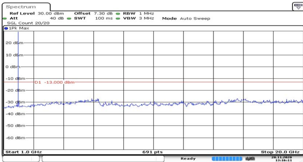
Channel 661 1GHz~20GHz
