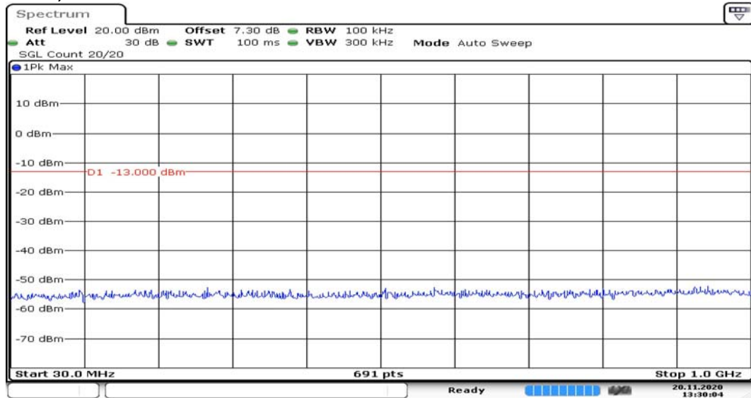
Channel 661 30MHz~1GHz
