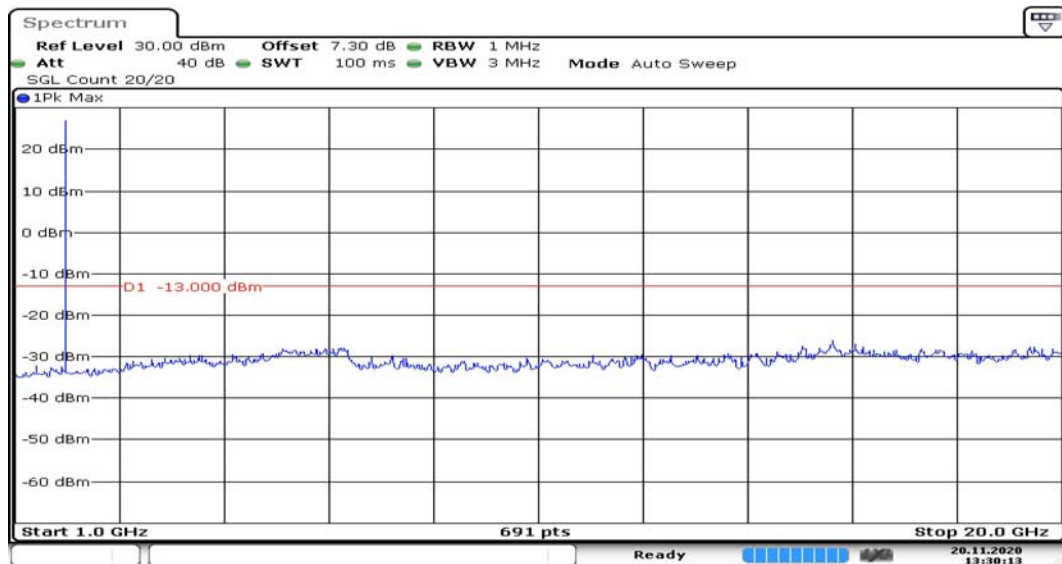
Channel 661 1GHz~20GHz
