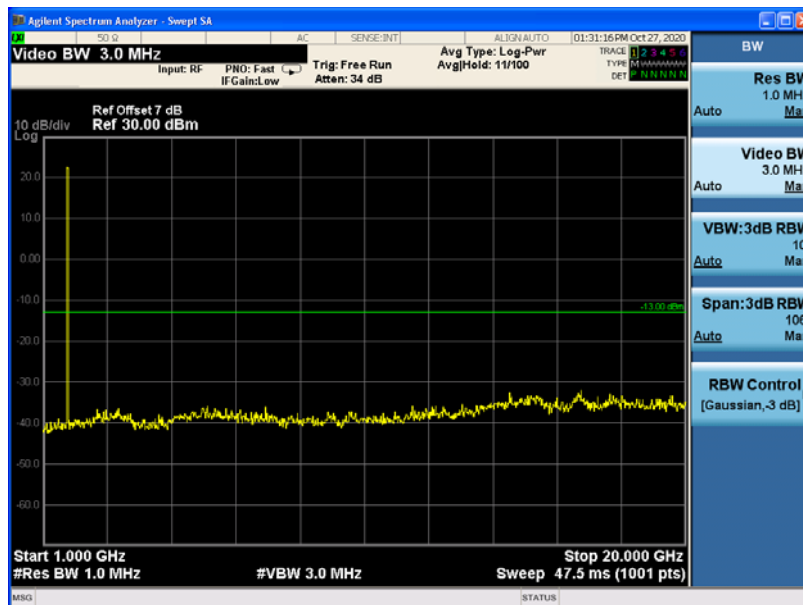
Channel 1412, 1GHz~20GHz
