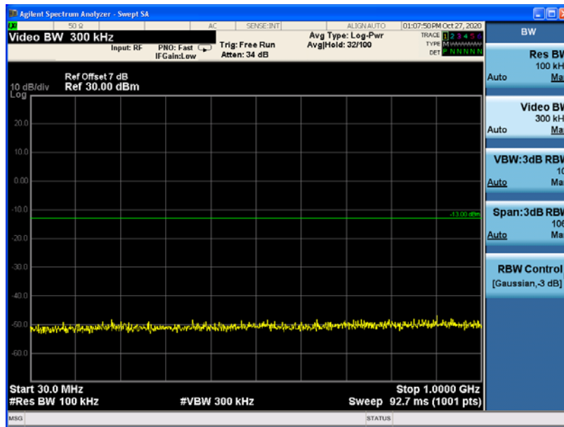
Channel 1412, 30MHz~1GHz
