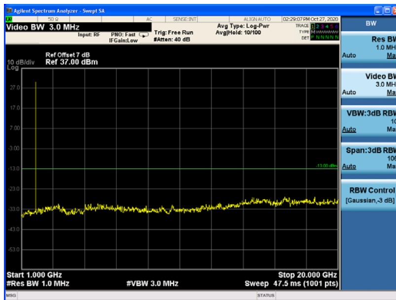
Channel 661, 1GHz~20GHz
