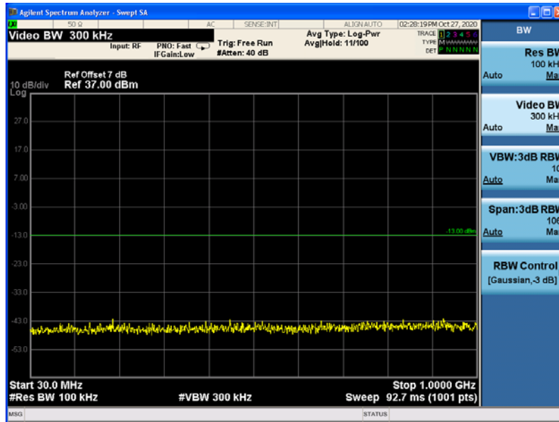
Channel 661, 30MHz~1GHz
