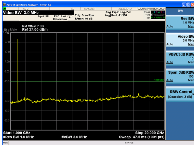
Channel 661, 1GHz~20GHz
