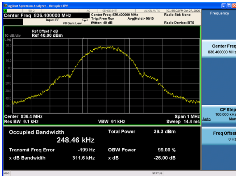
Channel 189
