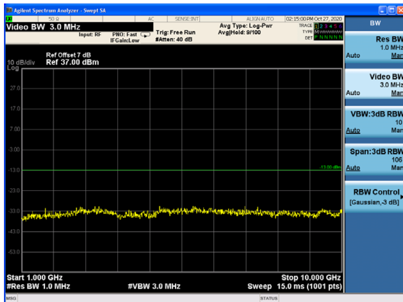
Channel 189, 1GHz~10GHz
