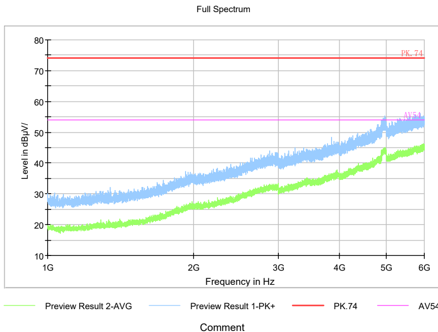
Pic12. Radiated emission (1GHz –6GHz)
