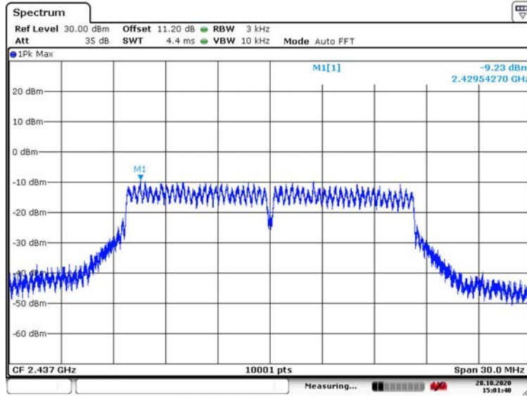
Carrier frequency (MHz): 2437 Channel No.6 Test Mode: 802.11g
