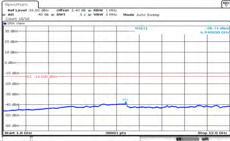
Band12-10MHz-16QAM-23060-1RB#0-Range2:1000~12000MHz
