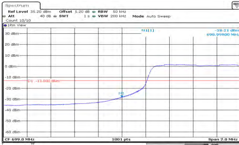
Band12-5MHz-16QAM-23035-25RB#0
