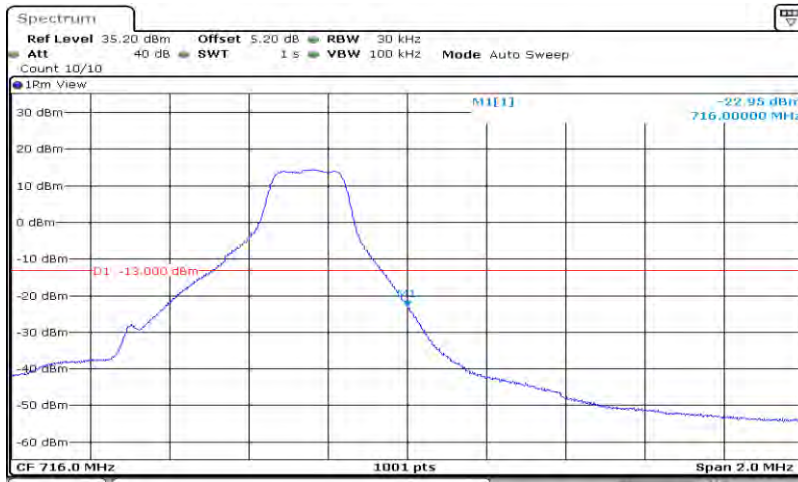
Band12-1.4MHz-16QAM-23173-6RB#0
