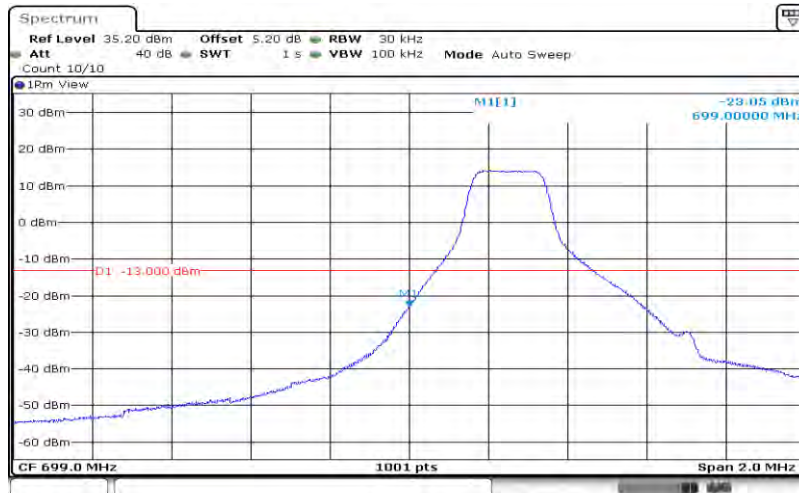
Band12-1.4MHz-16QAM-23017-6RB#0
