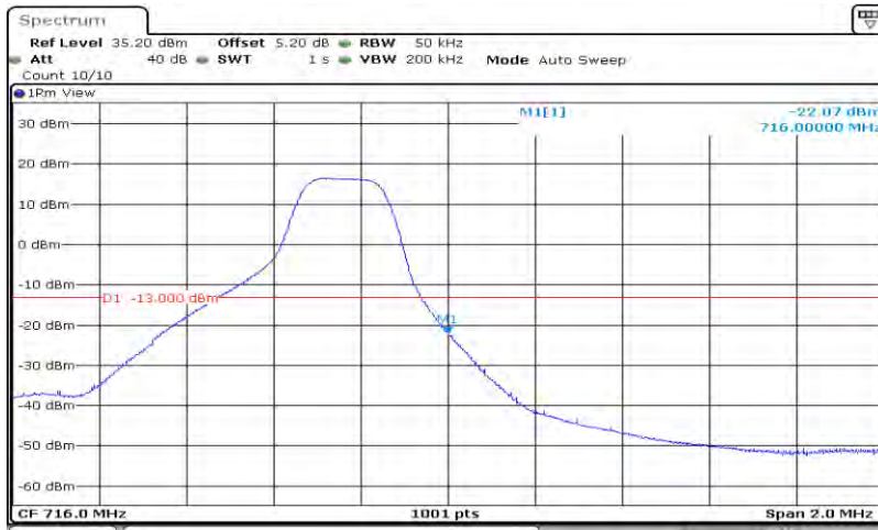
Band12-3MHz-16QAM-23165-15RB#0
