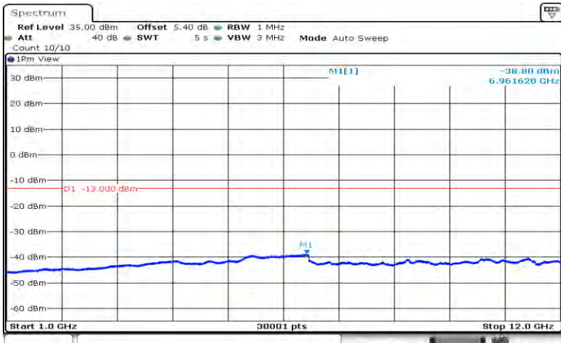
Band12-10MHz-16QAM-23095-1RB#0-Range2:1000~12000MHz
