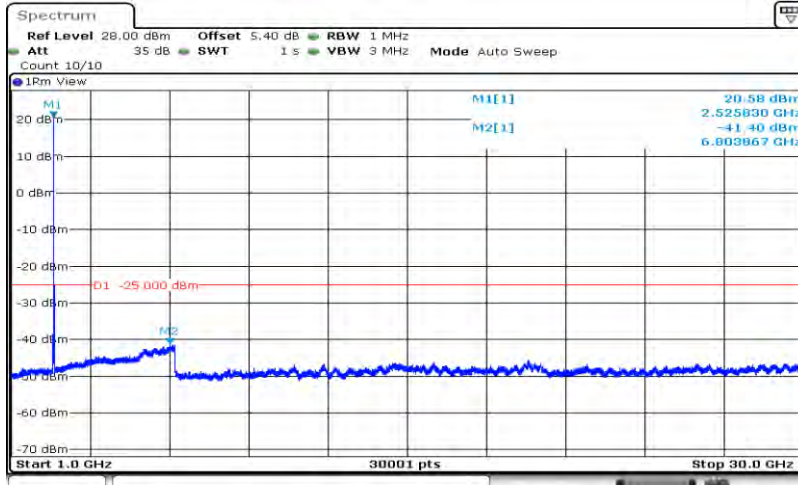
Band7-20MHz-16QAM-21100-1RB#0-Range2:1000~30000MHz
