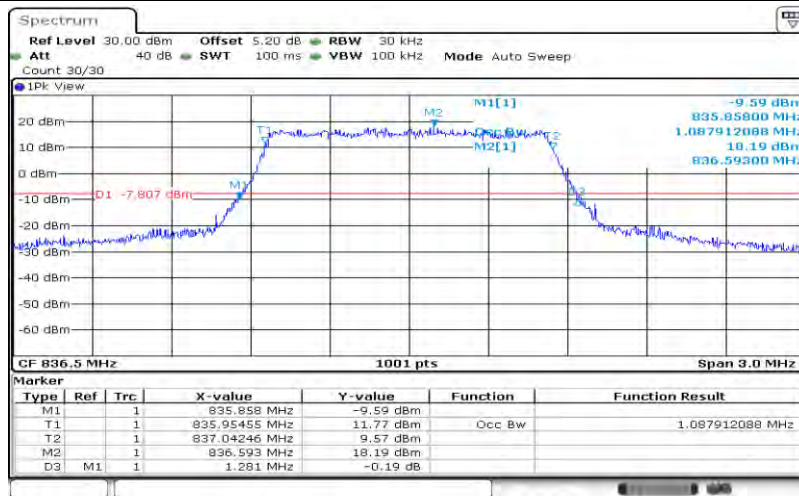
Band5-1.4MHz-QPSK-20525-6RB#0-1.088
