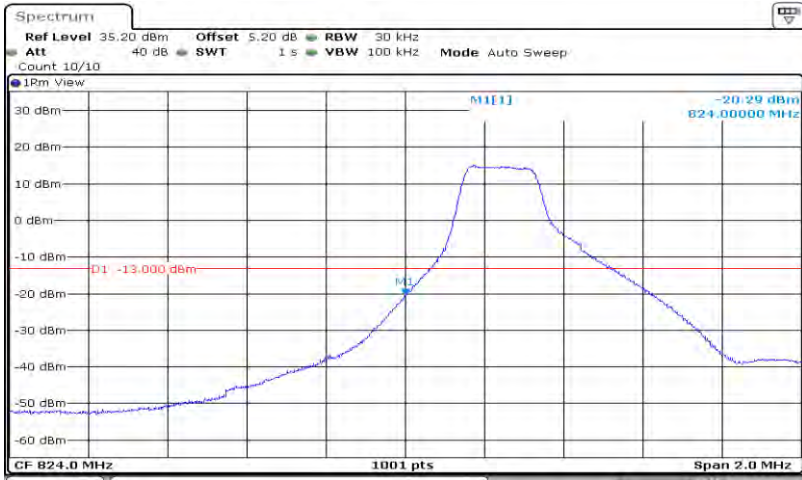
Band5-3MHz-16QAM-20415-15RB#0
