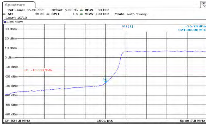
Band5-1.4MHz-16QAM-20407-6RB#0
