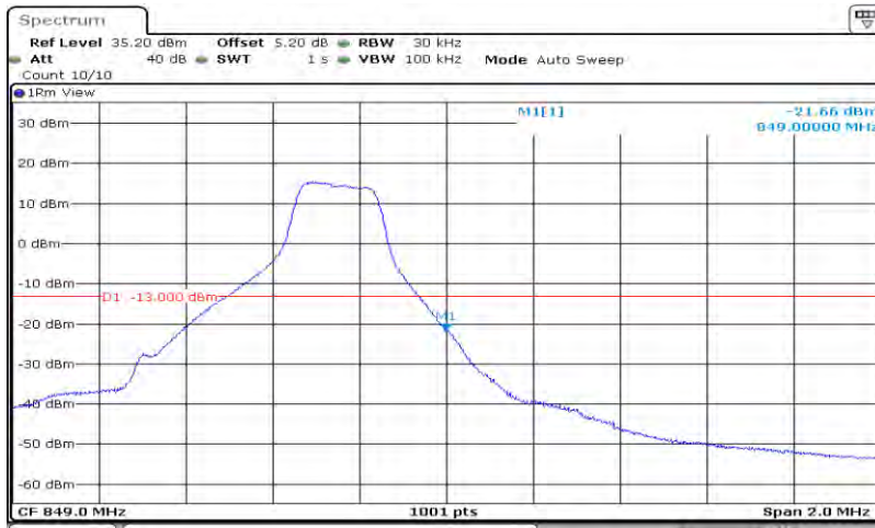
Band5-1.4MHz-16QAM-20643-6RB#0
