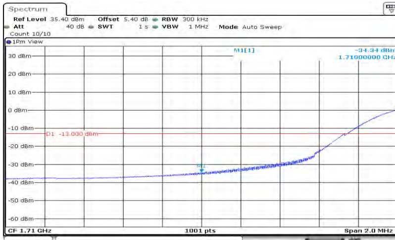
Band4-20MHz-16QAM-20050-100RB#0
