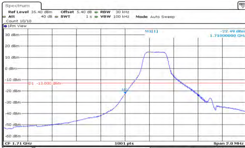
Band4-1.4MHz-16QAM-19957-6RB#0
