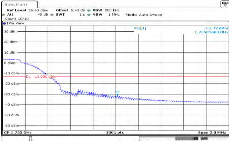
Band4-15MHz-QPSK-20325-75RB#0
