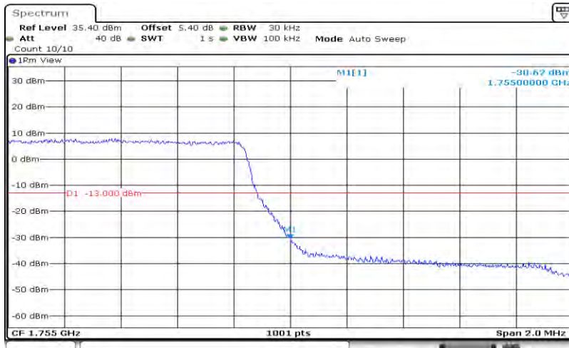
Band4-1.4MHz-QPSK-20393-6RB#0
