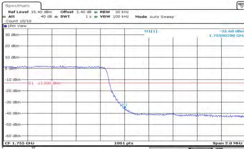
Band4-3MHz-16QAM-20385-15RB#0
