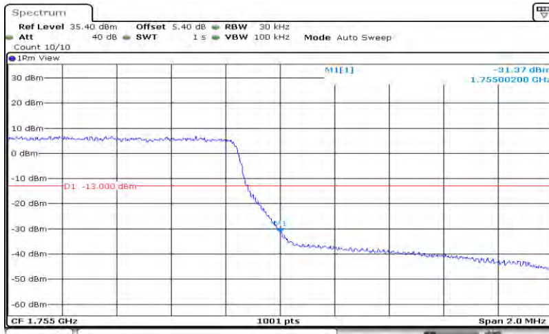
Band4-1.4MHz-16QAM-20393-6RB#0
