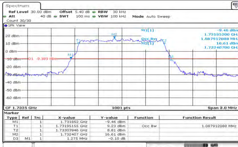
Band4-1.4MHz-QPSK-20175-6RB#0-1.088
