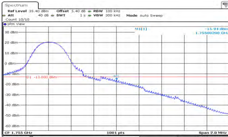
Band4-10MHz-QPSK-20350-50RB#0
