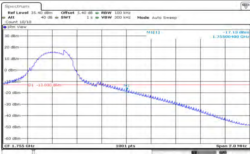
Band4-10MHz-16QAM-20350-50RB#0
