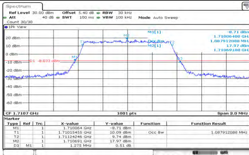
Band4-1.4MHz-QPSK-19957-6RB#0-1.088
