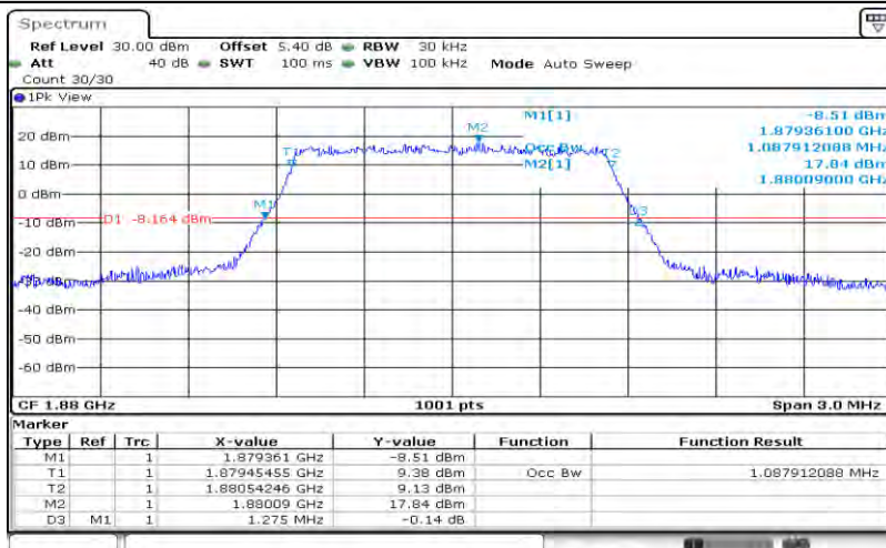
Band2-1.4MHz-QPSK-18900-6RB#0-1.088
