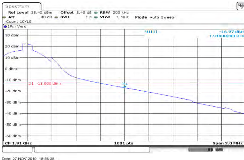
Band2-15MHz-QPSK-19125-75RB#0
