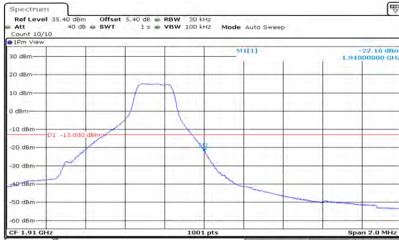
Band2-1.4MHz-16QAM-19193-6RB#0
