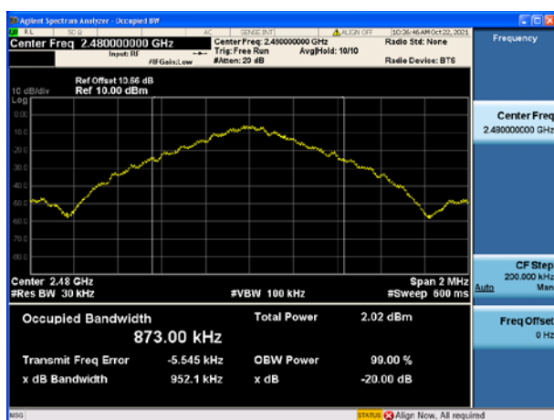
Modulation: GFSK 2480MHz
