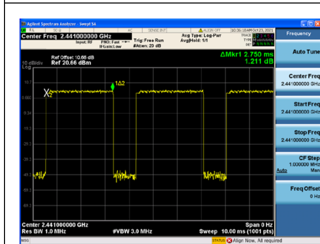
Modulation: 8DPSK 3DH5 2441MHz
