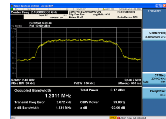
Modulation: 8DPSK 2480MHz
