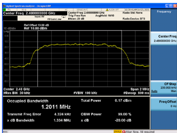
Modulation: 8DPSK 2480MHz
