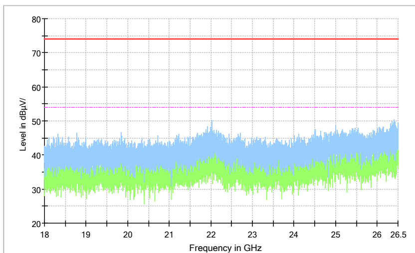
Full Spectrum
