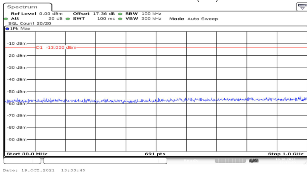
Channel 9400 30MHz~1GHz(dBm)
