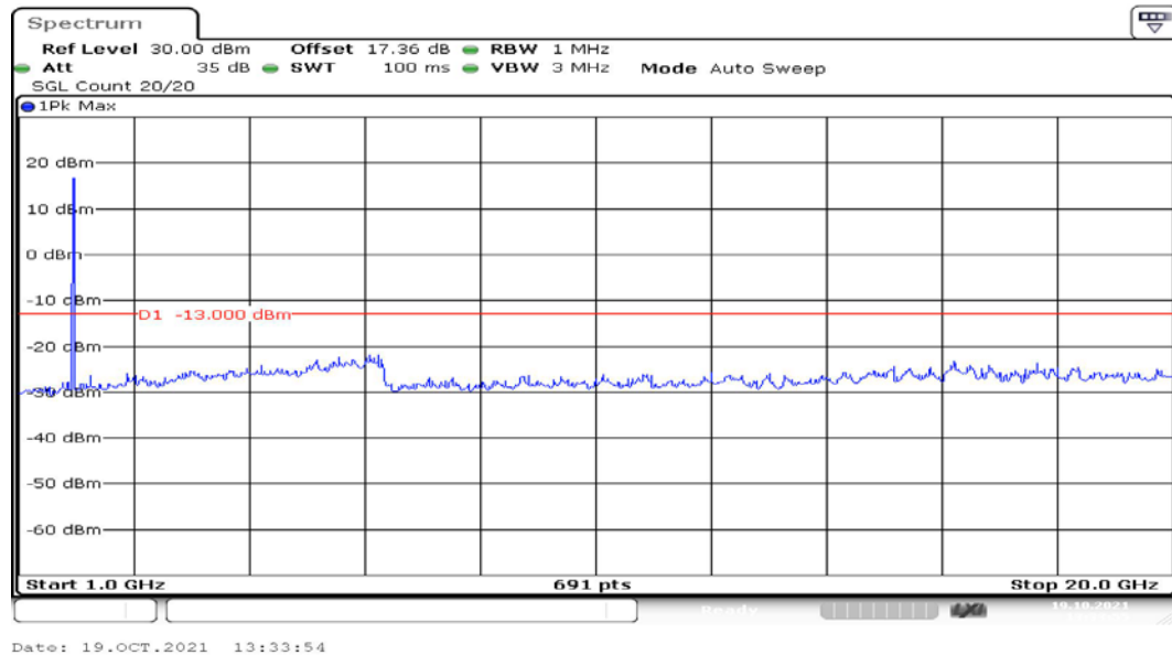
Channel 9400 1GHz~20GHz(dBm)
