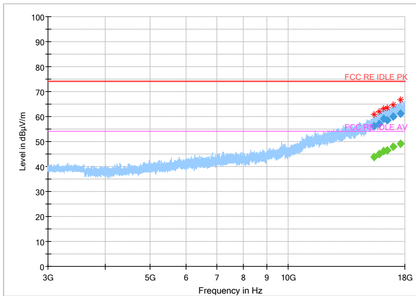
Fig.26 Radiated emission: Ch39, 3GHz~18GHz
