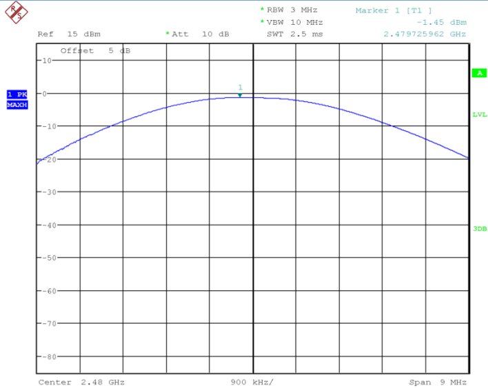
Fig.3 Peak Conducted Output Power CH39, DH1
