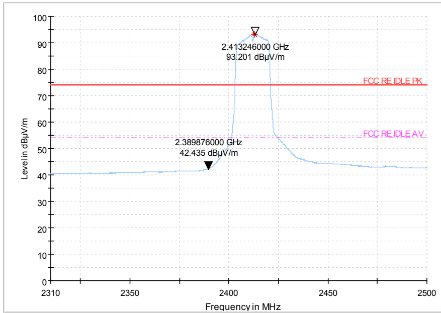
Fig.48 Radiated emission (Power): 802.11g, low channel
