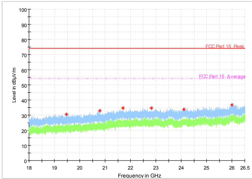
Fig. 32 Radiated Spurious Emission (802.11a, Ch165, 18 GHz-26.5 GHz)
