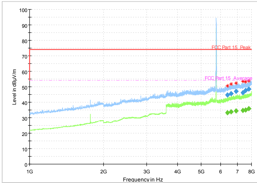
Fig. 34 Radiated Spurious Emission (802.11n-HT20, Ch149, 1 GHz-8 GHz)
