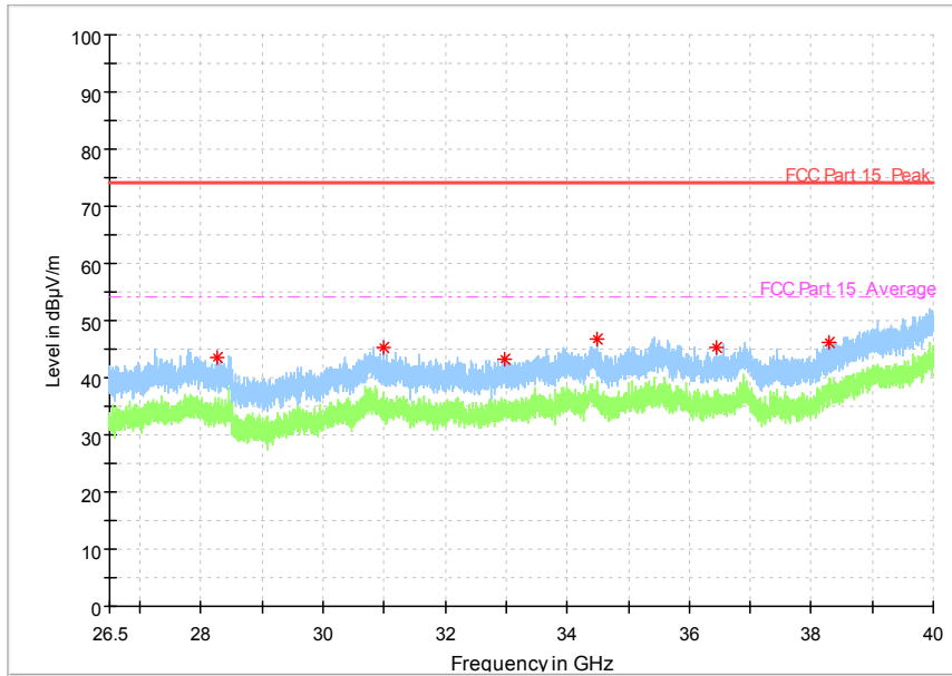
Fig. 42 Radiated emission: 802.11n, (802.11n-HT20, Ch165, 26.5 GHz - 40 GHz)
