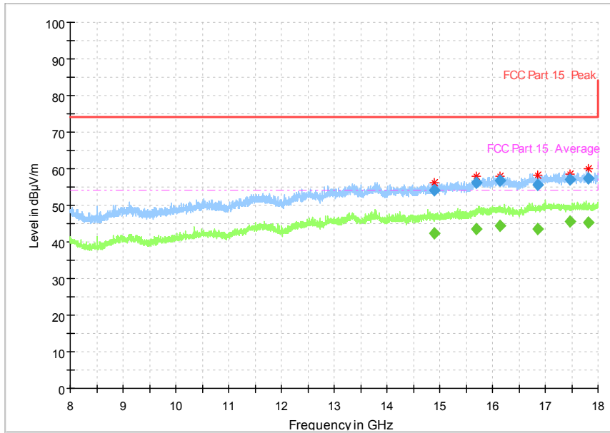
Fig. 26 Radiated Spurious Emission (802.11a, Ch149, 8 GHz-18 GHz)
