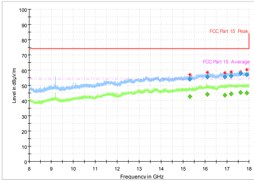
Fig. 40 Radiated Spurious Emission (802.11n-HT20, Ch165, 8 GHz-18 GHz)
