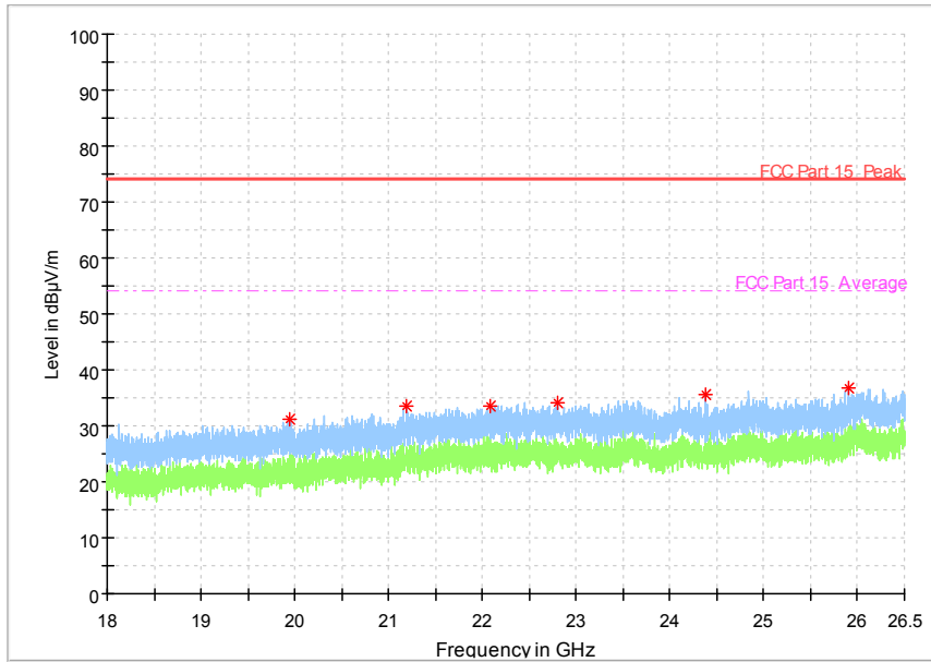
Fig. 46 Radiated Spurious Emission (802.11a, Ch149, 18 GHz-26.5 GHz)
