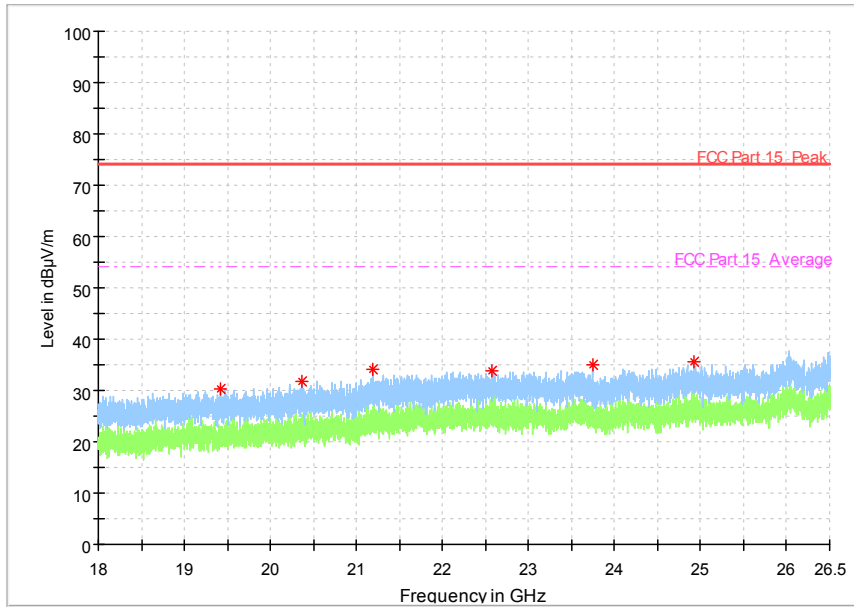
Fig. 56 Radiated Spurious Emission (802.11a, ch52, 18 GHz-26.5 GHz)
