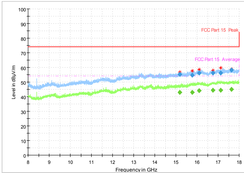
Fig. 50 Radiated Spurious Emission (802.11 n-HT20, ch64, 8 GHz-18 GHz)
