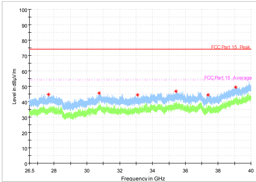
Fig. 52 Radiated Spurious Emission (802.11 n-HT20, ch64, 26.5 GHz-40 GHz)
