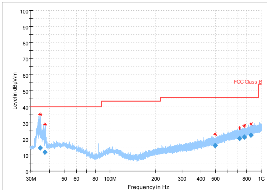
Fig. 53 Radiated Spurious Emission (802.11a, ch52, 30 MHz-1 GHz)
