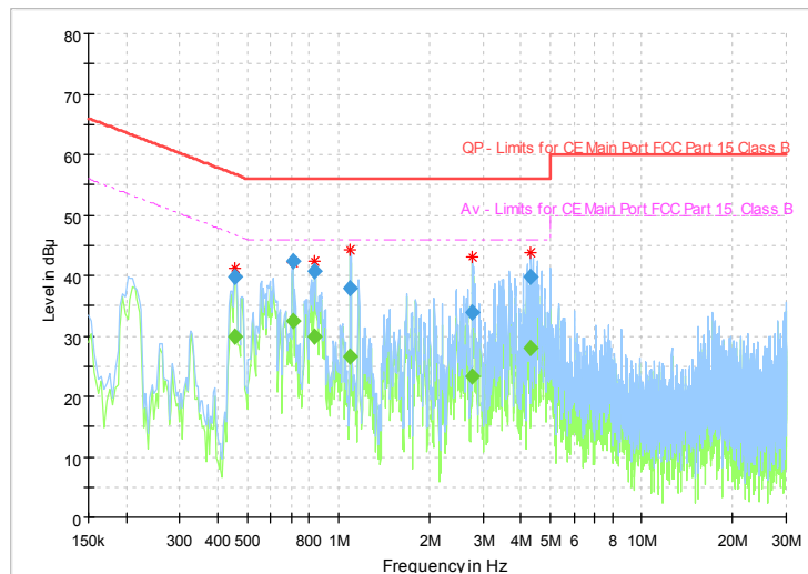
Fig.23AC Powerline Conducted Emission
