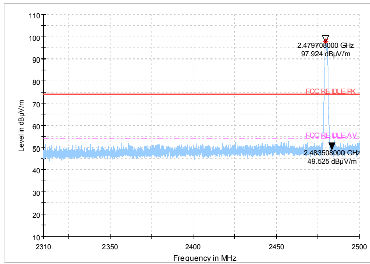
Fig.21 Bandedge PK:ch39
